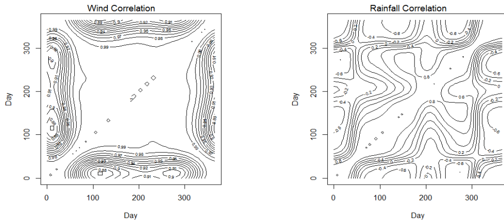
Figure 6 The contour plots of the bivariate correlation functions for wind and rainfall
