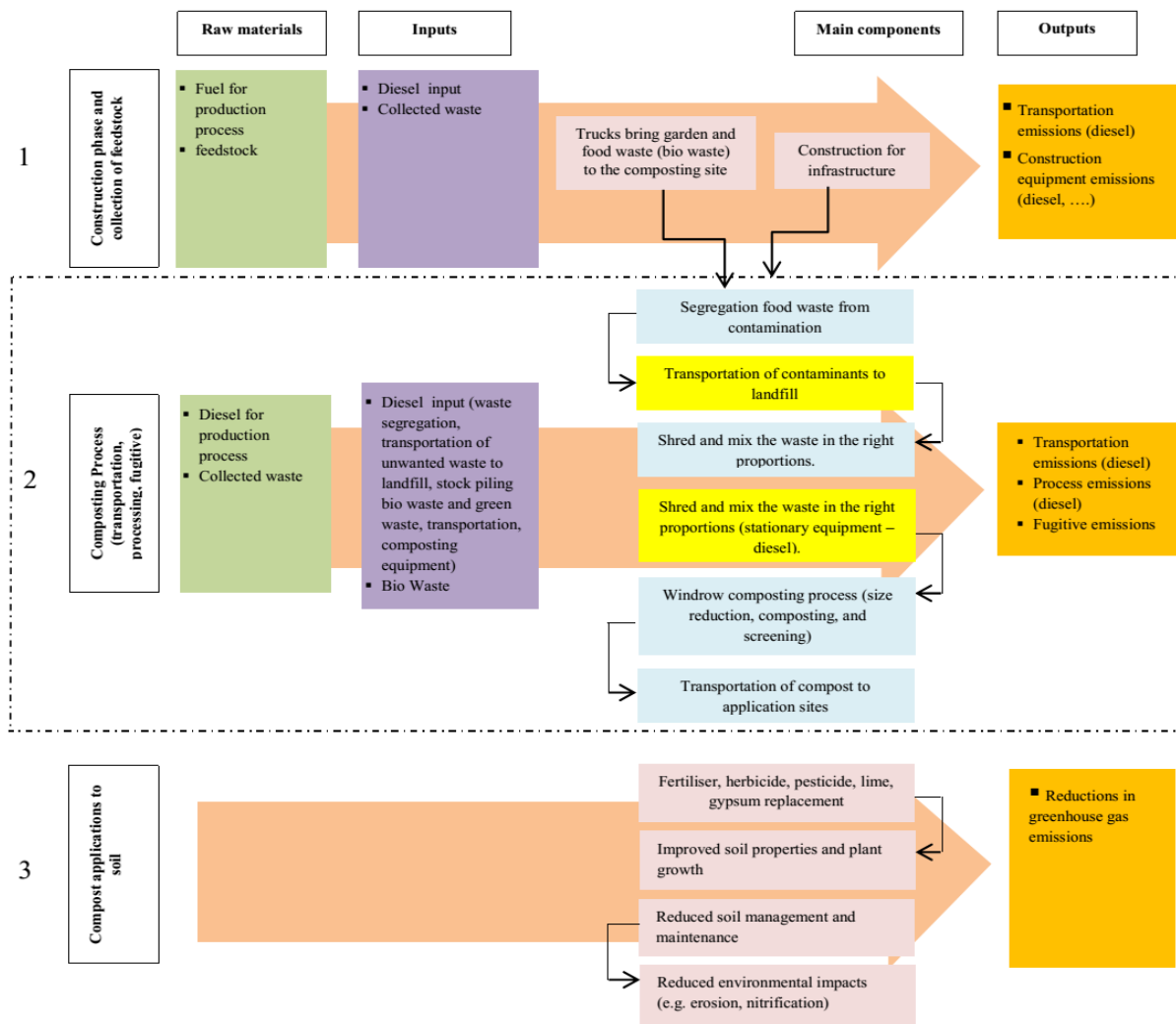
Figure 1 The framework for the calculation of GHGs emission during organic waste composting in UTM. The dashed line illustrates the scopes of the present study
