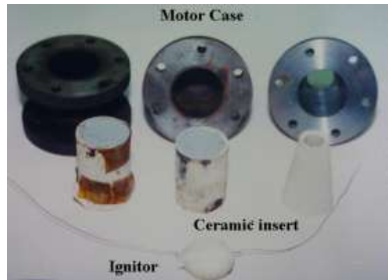
Figure 7 Ceramic insert with the rocket motor case and ignitor 9
