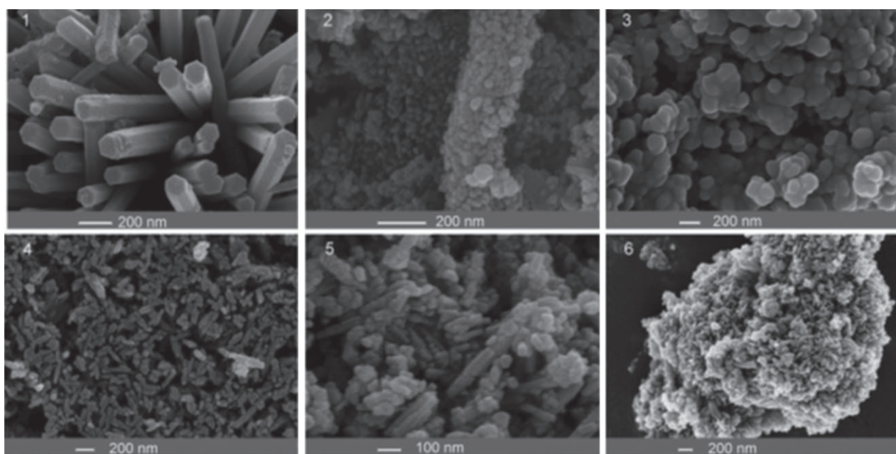
Figure 2 SEM images of ZnO nanostructures generated by ultrasound-assisted decomposition of Zn(OAc)_2 in (1) [C_4C_1Im][NTf_2] , (2) [C_8C_1Im][NTf_2] , (3) [C_{10}C_1Im][NTf_2] , (4) [C_4C_1Im][NTf_2] , (5) [N_{1,1,4}][NTf_2] , and (6) [C_4C_1Im][SCN] . © Wiley-VCH [67].
