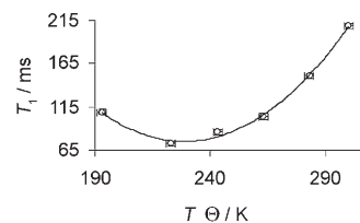
Figure 6. T_1 values as a function of temperature determined for [Ru(dtbpmp)H 2 (H 2 )] 6 . T_1/\text{ms} ( \Delta 3 ms) [ T/\text{K} ( \Delta 2 K)]: 209 [300], 151 [283], 104 [263], 86 [243], 73 [223], 109 [193].
