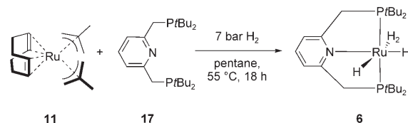
Scheme 4. Direct hydrogenation of [Ru(cod)(metallyl) 2 ] ( 11 ) in the presence of dtbpmp ( 17 ) to give the nonclassical ruthenium hydride complex 6 .
