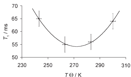
Figure 3. Temperature-dependent evolution of the T_1 values measured for 4a . T_1/\text{ms} ( \Delta 3 ms) [ T/\text{K} ( \Delta 2 K)]: 64 [300], 56 [283], 55 [263], 65 [243], 108 [223].
