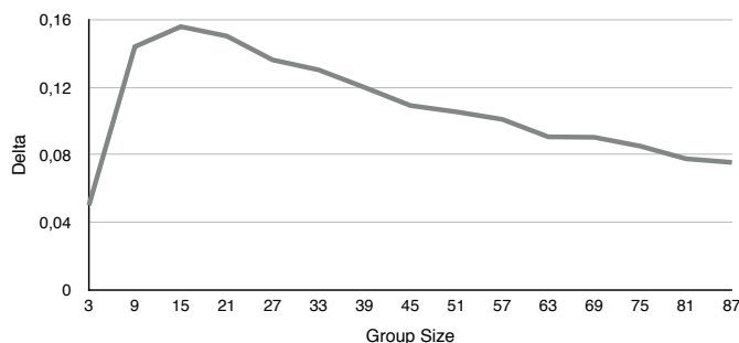
Figure 7: \Delta for a group with only one highly reliable member. One member has a reliability of 0.9, the rest has a reliability of 0.55. The (initial) second order reliability is 0.85.
