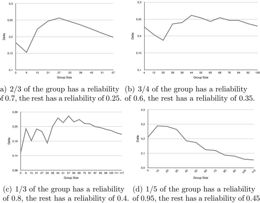
Figure 4: \Delta as a function of the group size.
