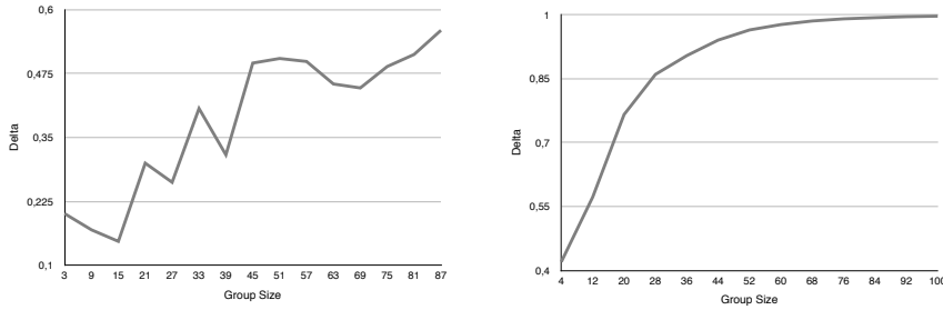
(a) 1/3 of the group has a reliability of 0.75, the rest has a reliability of 0.25. (b) 1/4 of the group has a reliability of 0.8, the rest has a reliability of 0.25.
