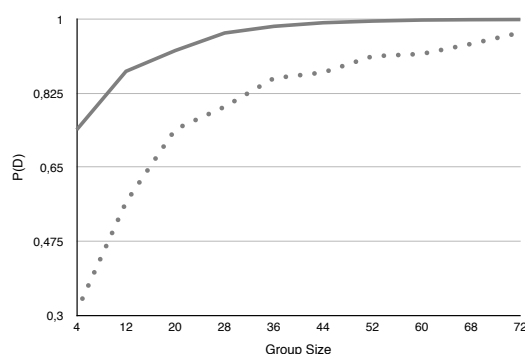
Figure 3: P_D for inhomogeneous groups as a function of the group size. (a) 1/4 of the group members has a reliability of 0.25, the rest has a reliability of 0.7 (solid line). (b) 1/4 of the group members has a reliability of 0.7, the rest has a reliability of 0.25 (dotted line).
