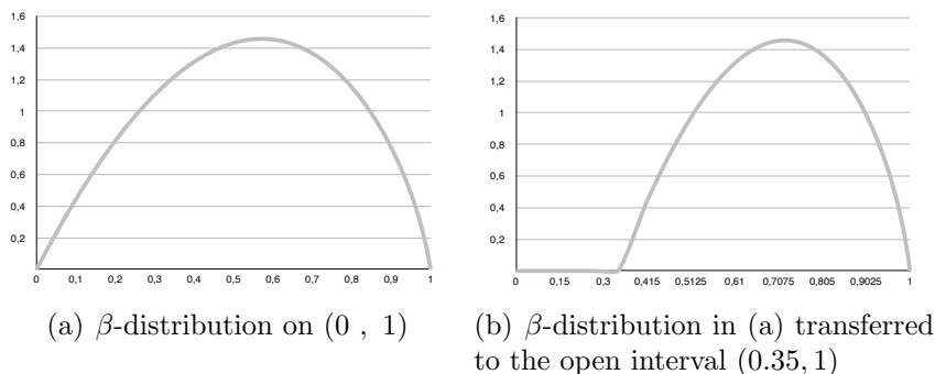
Figure 1: The \beta -distribution with parameters \alpha = 2 and \beta = 1.625 corresponding to r_j = 0.75 and c_i = 0.6 .
