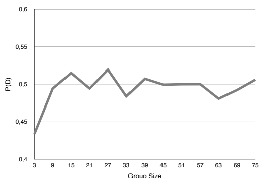
Figure 2: P_D for a homogeneous group as a function of the group size. Each group member has a reliability of 0.4.
