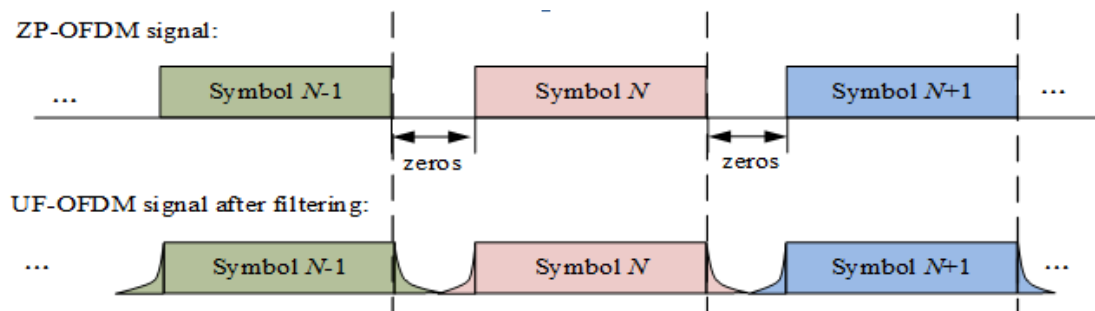
FIGURE 4.2: UFMC Symbol [17]
