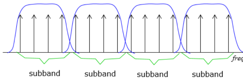
FIGURE 4.1: Subband Filtering
