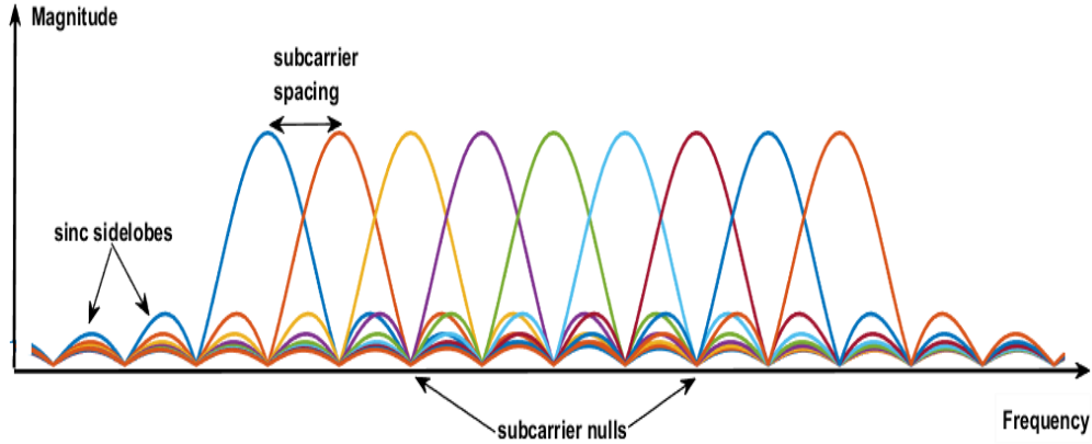
FIGURE 2.7: OFDM spectrum
