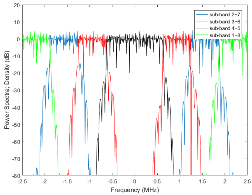
FIGURE 4.4: UFMC inBand Spectrum
