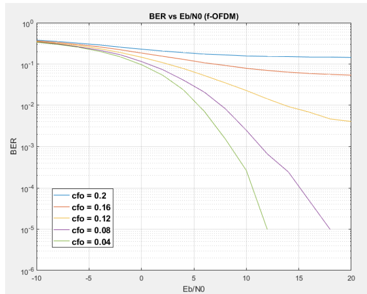
FIGURE 5.4: f-OFDM performance in presence of CFO
