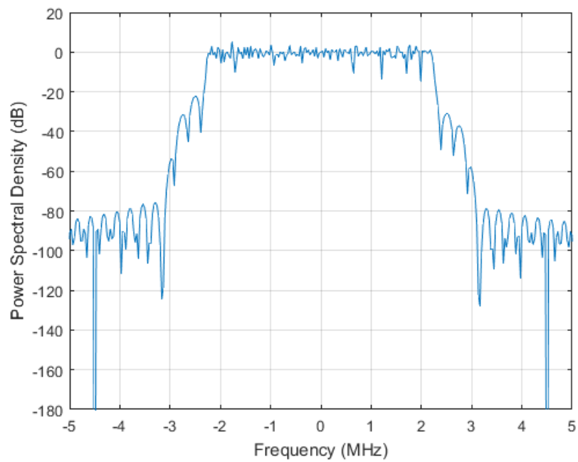
FIGURE 4.5: UFMC Spectrum
