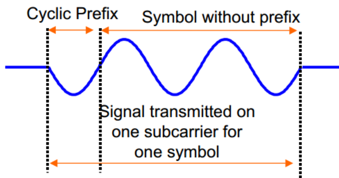
FIGURE 2.5: CP Insertion
