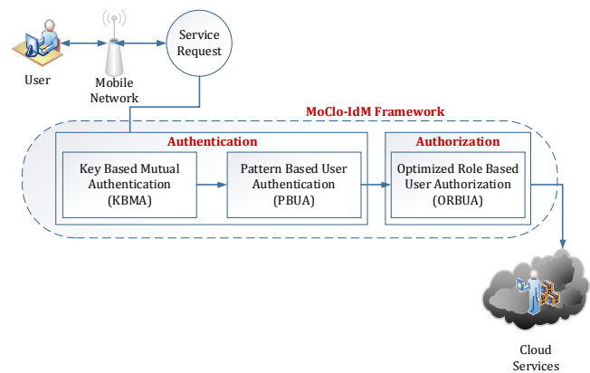
Fig. 2 Workflow of MoClo-IdM Framework
