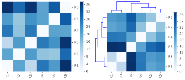
Figure 5: Distance matrix of temperature movements with Euclidean distance (left) and agglomerative clustering clustergram of temperature readings for six rooms with Ward (right).
