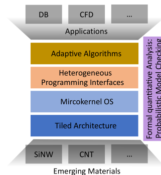
Fig. 1. The Orchestration Stack
