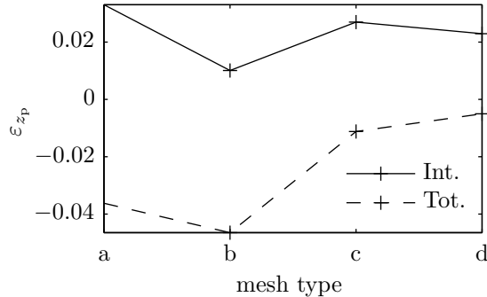
Figure 14: Results for the pure bending test: relative error \varepsilon_{z_p}(t=1) defined in Eq. (45) for various meshes depicted in Fig. 10. "Int." relates to interpolation (exact summation rule) and "Tot." to interpolation plus summation (central summation rule).
