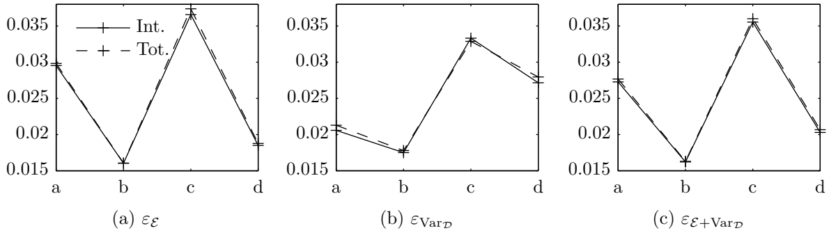
Figure 20: Results for the indentation test: relative errors \varepsilon_{\square} defined in Eq. (40) for the various meshes depicted in Fig. 16. "Int." relates to interpolation (exact summation rule) and "Tot." to interpolation plus summation (central summation rule).
