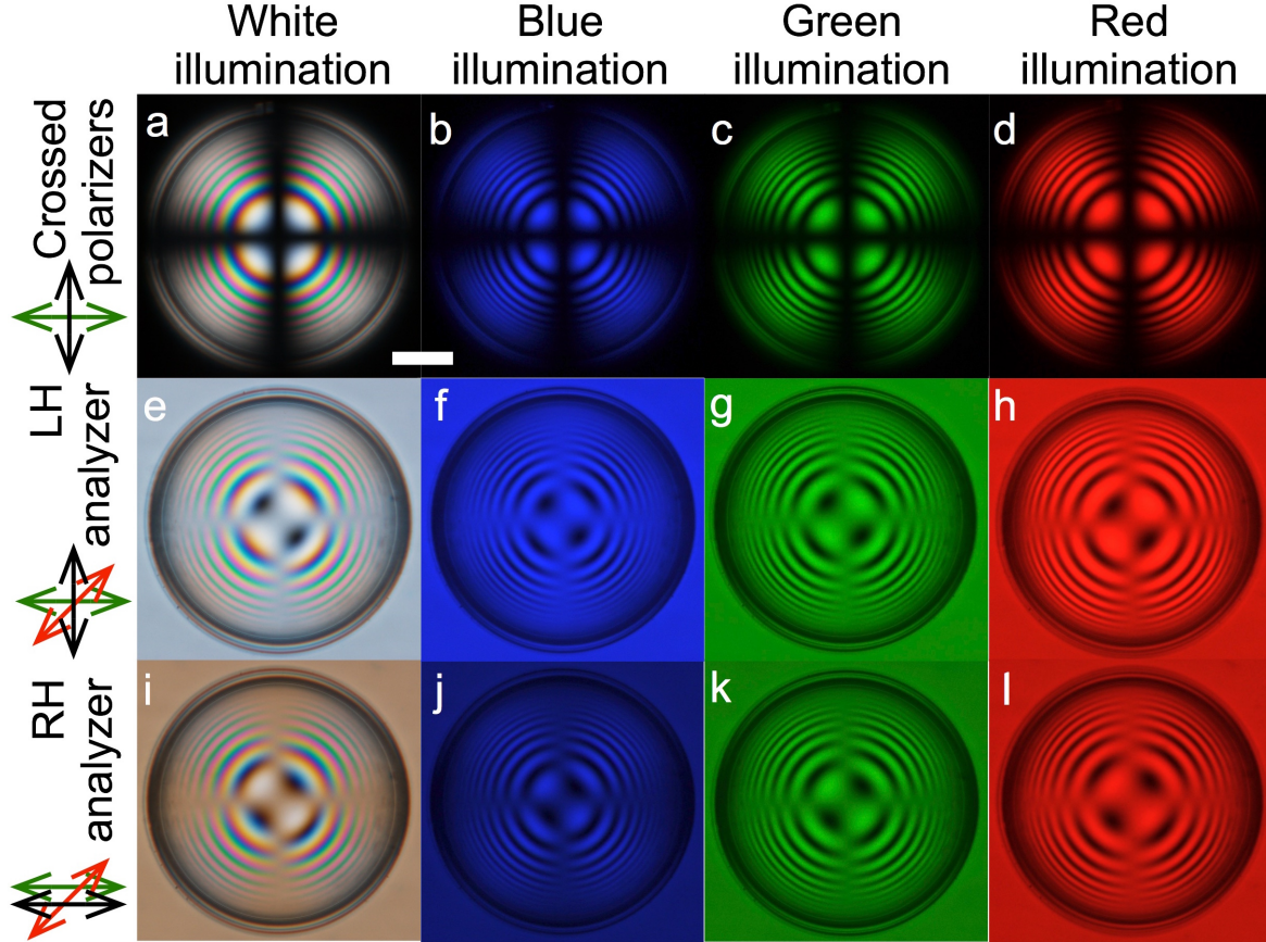
Figure 4. A shell of the non-chiral liquid crystal 5CB, in the nematic state with homeotropic alignment. The arrangement of panes is identical to that in Fig. 3. The scale bar is 50 \mu\text{m} .
