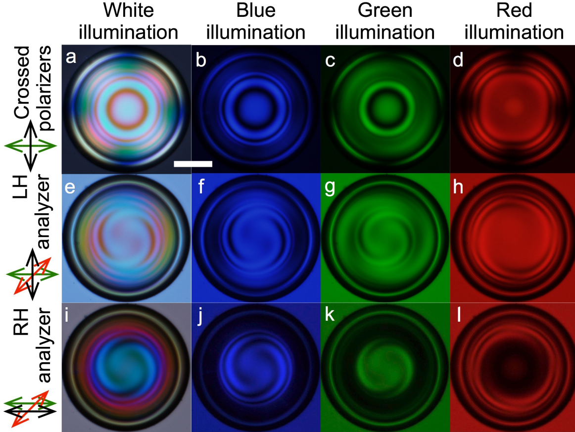
Figure 5. An isolated thick planar-aligned shell of the same liquid crystal as in Fig. 2 and Fig. 3. The arrangement of panes is identical to that in Fig. 3. The scale bar is 50 \mu\text{m} .
