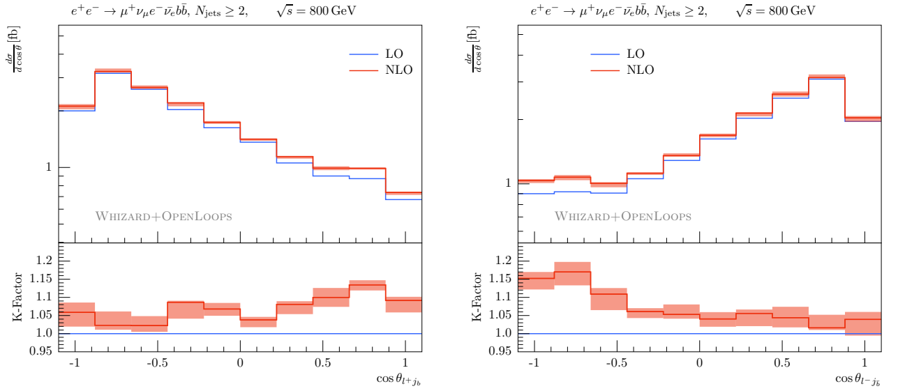
Figure 20: Distributions differential in the angular separations \cos\theta_{\ell+j_b} (left) and \cos\theta_{\ell-j_b} (right) for e^+e^- \rightarrow \mu^+\nu_\mu e^-\bar{\nu}_e b\bar{b} . Curves and bands as in Fig. 10.
