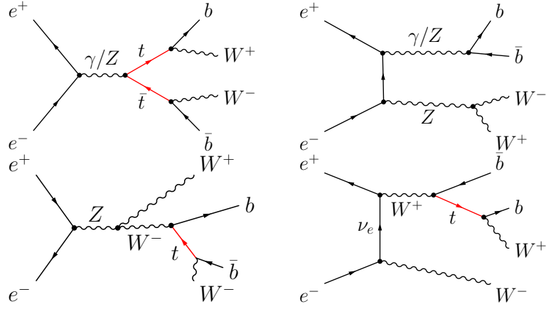
Figure 2: The double-resonant signal diagram (top left) besides example non-resonant (top right) and s - and t -channel single-top diagrams (bottom left and right, respectively) of the process e^+e^- \rightarrow W^+W^-b\bar{b} .
