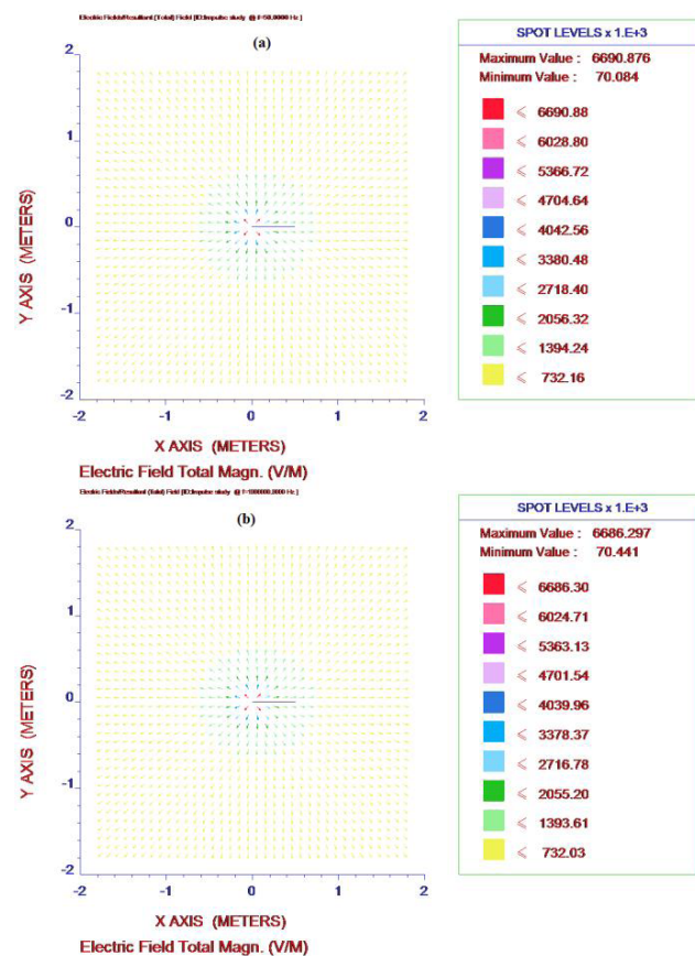
FIGURE 9. Electric field distribution at earth surface at a lightning incident at 50 Hz frequency (a) and at 1 MHz frequency (b).
