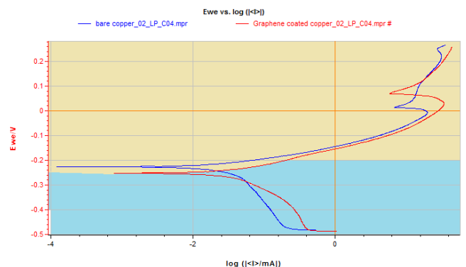
FIGURE 5. Polarization curves of the graphene-coated and uncoated copper in 0.1 M sodium chloride solution. (Light yellow indicates the anodic region and light turquoise the cathodic region of the plots.) As the intercept point of anodic and cathodic plots has shifted to the positive direction it could be reported that the graphene-coated copper conductor will be less susceptible to corrosion than the uncoated copper.
