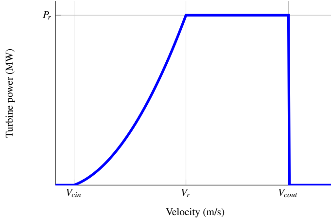
Fig. 5 The turbine power curve with maximum production p_r = 6 MW
