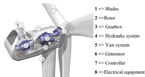
Fig. 1 Crucial subsystem of an offshore wind turbine, based on [16]
