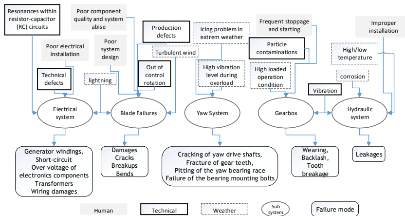
Fig. 2 Principal cause of turbine failure
