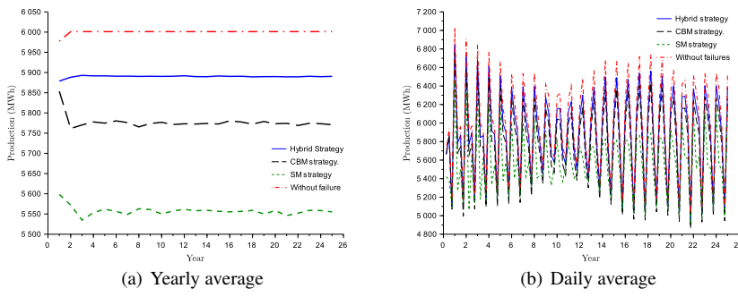
Fig. 12 Electricity production variation over 25 years
