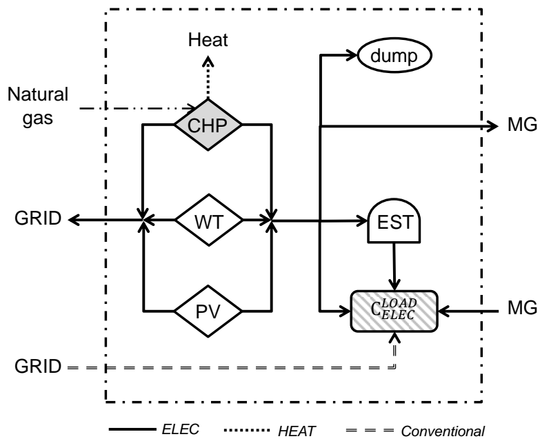
(a) Black-box diagram electricity supply alternatives
