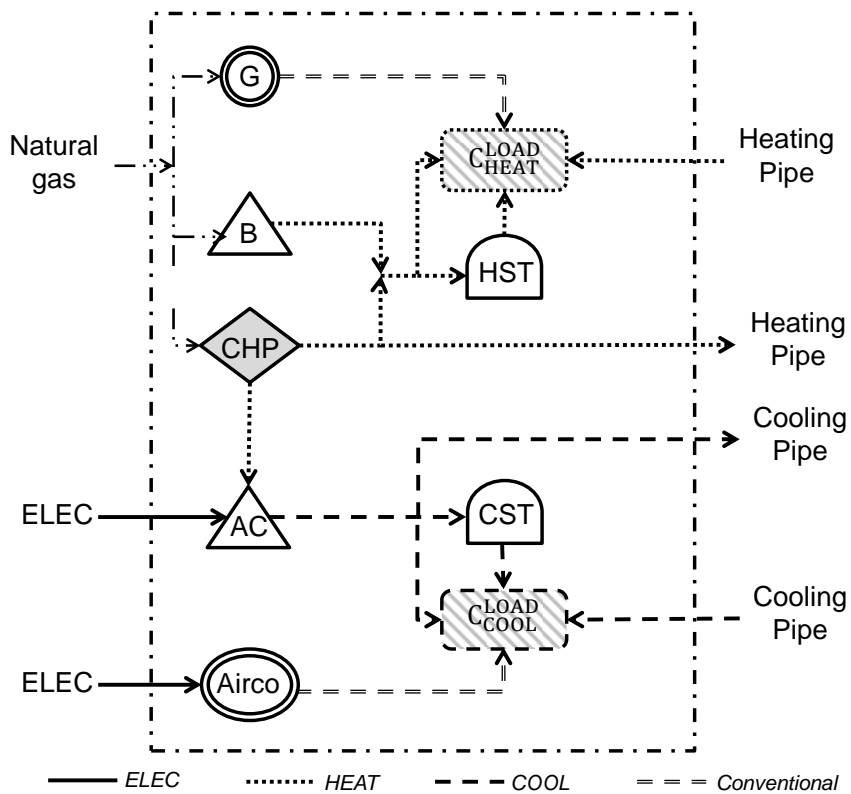
(b) Black-box diagram heating and cooling supply alternatives
