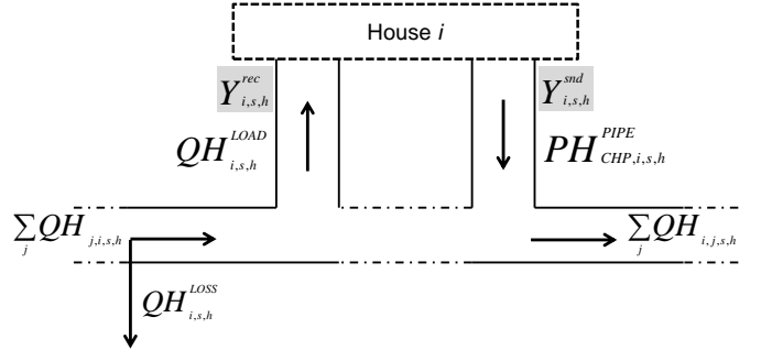
Figure 2: Schematic of pipeline operation of house i . Grey=Binary variable.
