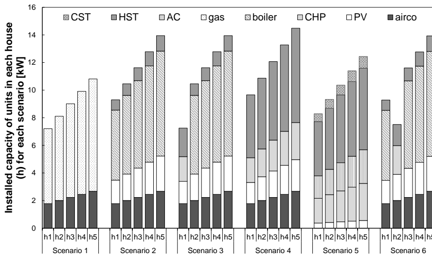
(a) Installed units (kW) in each household (h) for each scenario
