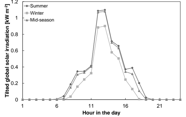
(a) Daily profiles of hourly averaged tilted global solar irradiation for a typical day in each season (kW m^{-2} )
