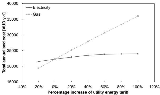
Figure 10: Total annualised cost versus percentage increase of utility energy tariffs of electricity and gas [AUD y^{-1} ].
