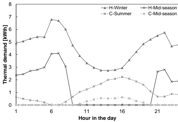
(b) Thermal demand for a typical day in each season. C=space cooling, H=space heating
