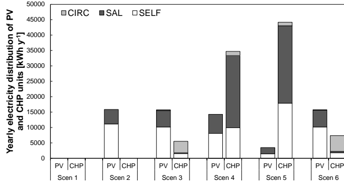
Figure 7: Summary of the yearly electricity distribution [ \text{kWh y}^{-1} ] of all the PV and CHP units in the neighbourhood for each scenario.
