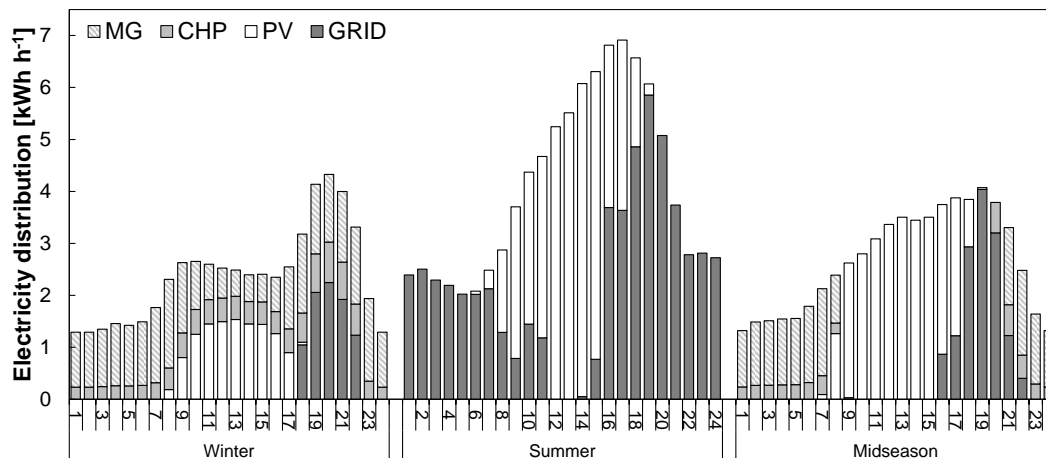
Figure 6: Neighbourhood electricity supply distribution to meet total local demand for a typical day (24 hours) in each season [kWh h -1 ], scenario 6. Note that the summer electricity demand includes cooling through air-conditioning systems.
