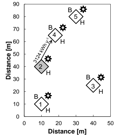
(b) Neighbourhood lay-out, Scenario 6
