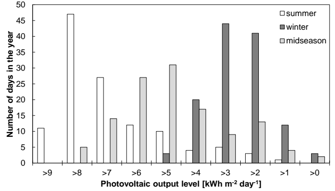
Figure 11: Occurrence rate of different daily PV output levels in each season [kWh m^{-2} day^{-1} ].
