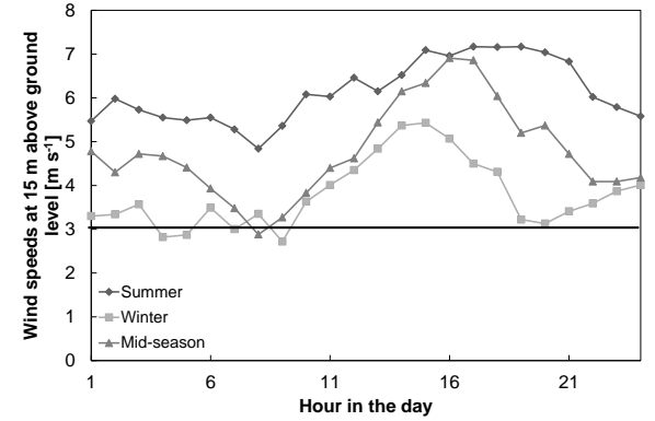
(b) Daily profiles of hourly averaged wind speeds at 15 m above ground level for a typical day in each season (m s^{-1} ). The horizontal line indicates the cut-in wind speed of the turbines
