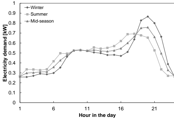
(a) Electricity demand for a typical day in each season, including lighting and household appliances but excluding cooling requirements
