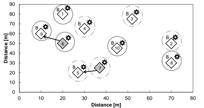
Figure 9: Lay-out of the neighbourhood with 10 houses and multiple MGs. All houses have air-conditioning, heat storage and PV units installed. Diamonds=houses, grey diamond=CHP unit, sun=PV unit, arrow=heating pipeline connection, dashed circles=pools.
