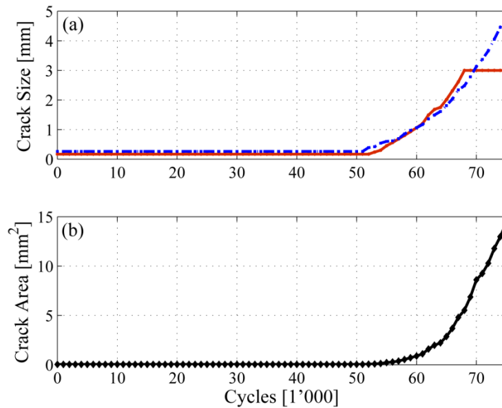
Figure 4. Typically observed fatigue crack growth for same specimen as photos in Fig. 3; (a) optically measured crack length on specimen surface (dash-dotted) and crack depth in fastener hole interior (solid); (b) calculated crack area; shown against number of cycles.
