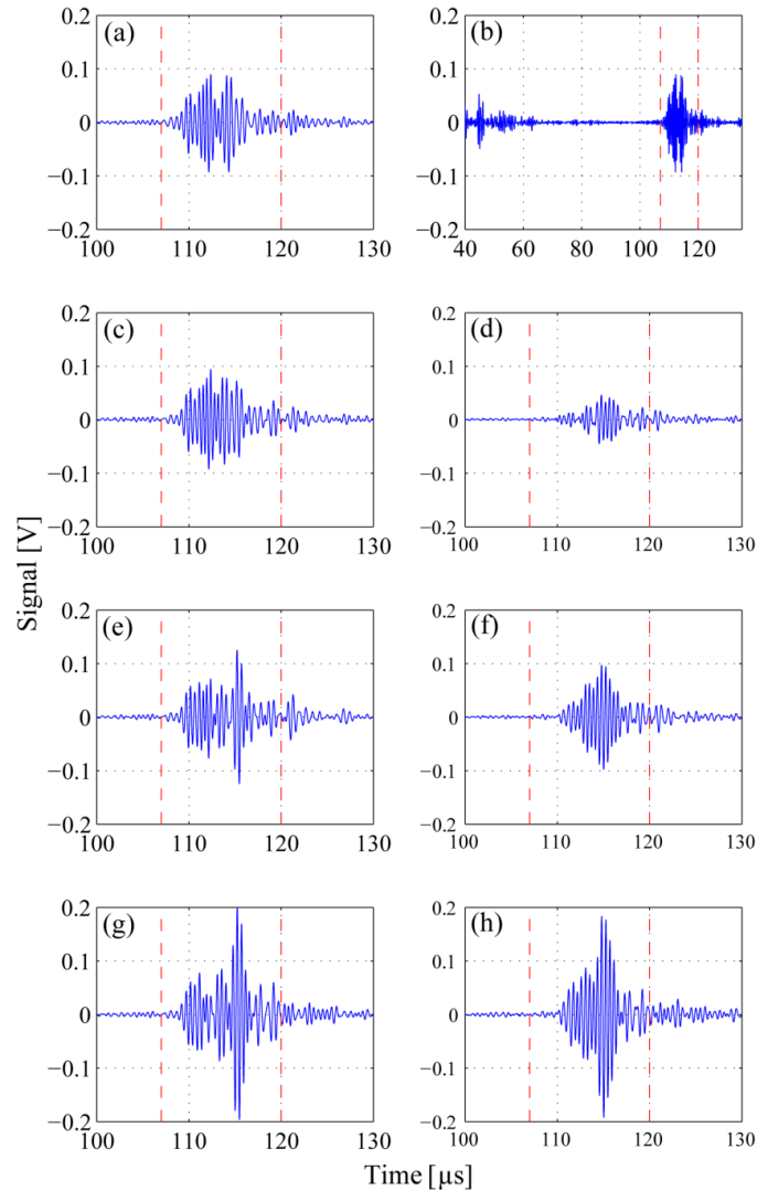
Figure 5. Measured P/E time traces and baseline subtracted signal differences (time window 107 – 120 \mu\text{s} shown); (a) zoom of signal for 10'000 cycles, no crack (baseline); (b) signal for 10'000 cycles; (c) signal for 60'000 cycles, crack length 1.06 mm, crack depth 1.06 mm; (d) signal difference for 60'000 cycles; (e) signal for 65'000 cycles, crack length 1.81 mm, crack depth 2.01 mm; (f) signal difference for 65'000 cycles; (g) signal for 70'000 cycles, crack length 3.13 mm, through thickness; (h) signal difference for 70'000 cycles.
