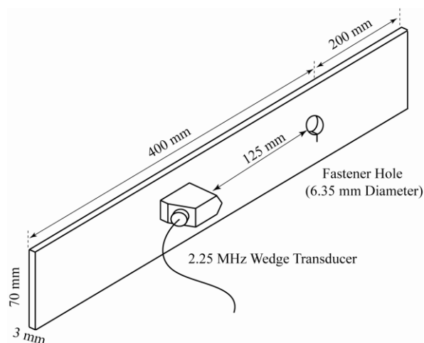
Figure 2. Schematic of tensile specimen (Al 2014 T6, 600 mm x 70 mm x 3 mm) with fastener hole (1/4 in / 6.35 mm diameter) and location of 2.25 MHz wedge transducer.
