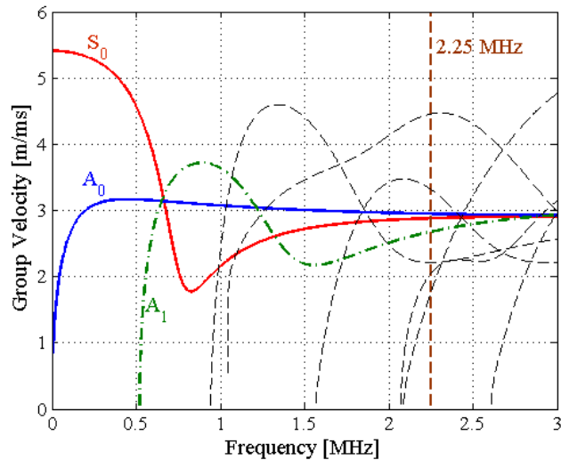
Figure 1. Group velocity dispersion diagram for 3 mm thick aluminum plate (Al 2014 T6); fundamental modes ( A_0 and S_0 ): solid lines; A_1 mode: dash-dotted line; higher order modes: dashed lines; center frequency 2.25 MHz marked.
