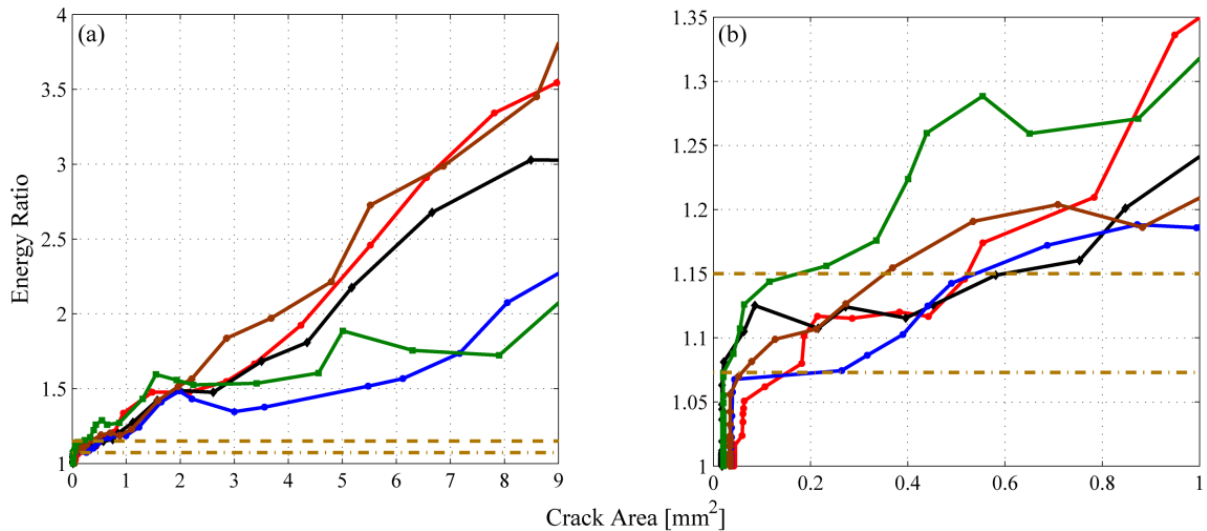
Figure 6. (a) Energy ratio of reflected P/E signal for 5 tensile specimens against optically measured crack area (solid lines); time window 107 – 120 \mu\text{s} ; (b) zoom for small crack area; 7.3% maximum variation before visual crack observation (dash-dotted); 15% threshold (dashed).
