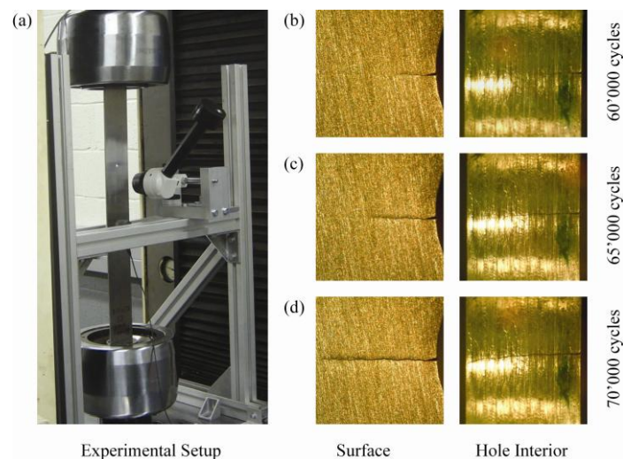
Figure 3. (a) Photo of tensile specimen in hydraulic testing machine with microscope and transducer; photos of crack on specimen surface (left) and through hole interior (right): (b) 60'000 cycles, crack length 1.06 mm, crack depth 1.06 mm; (c) 65'000 cycles, crack length 1.81 mm, crack depth 2.01 mm; (d) 70'000 cycles, crack length 3.13 mm, through thickness.
