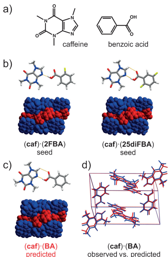
Figure 10. a) Molecular structure of caffeine ( caf ) and benzoic acid ( BA ). b) Cocrystals as heteronuclear seeds: cocrystals composed of caffeine ( caf ), 2-fluorobenzoic acid ( 2FBA ), and 2,5-difluorobenzoic acid ( 25diFBA ). c) Predicted lowest-energy crystal structure of ( caf )·( BA ). d) Overlay of the isomorphous lowest-energy predicted and obtained ( caf )·( BA ) cocrystal (red: predicted, blue: observed).
