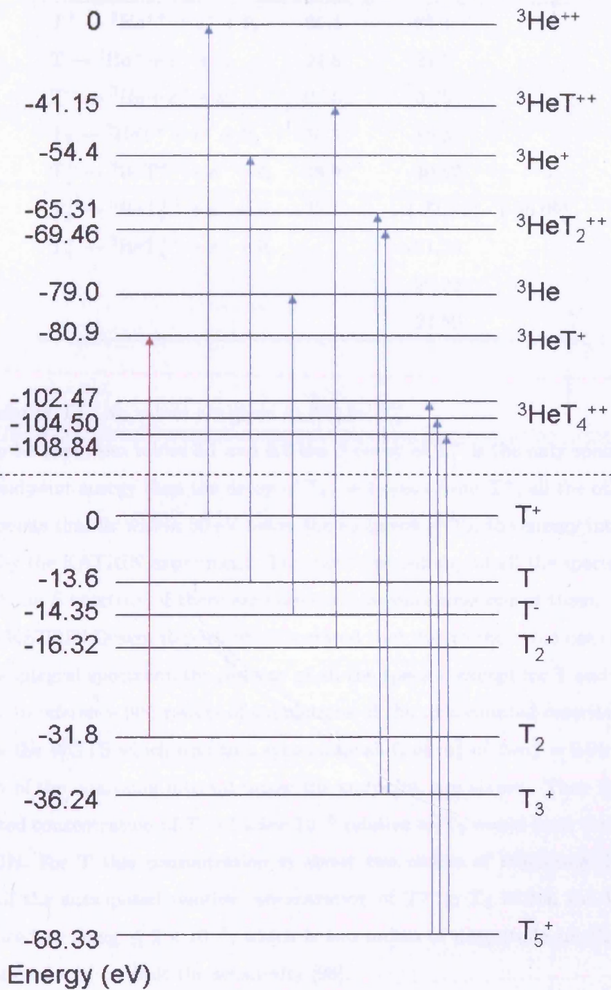
Figure 8.6: Ground state energies of the tritium species. See text for details.
