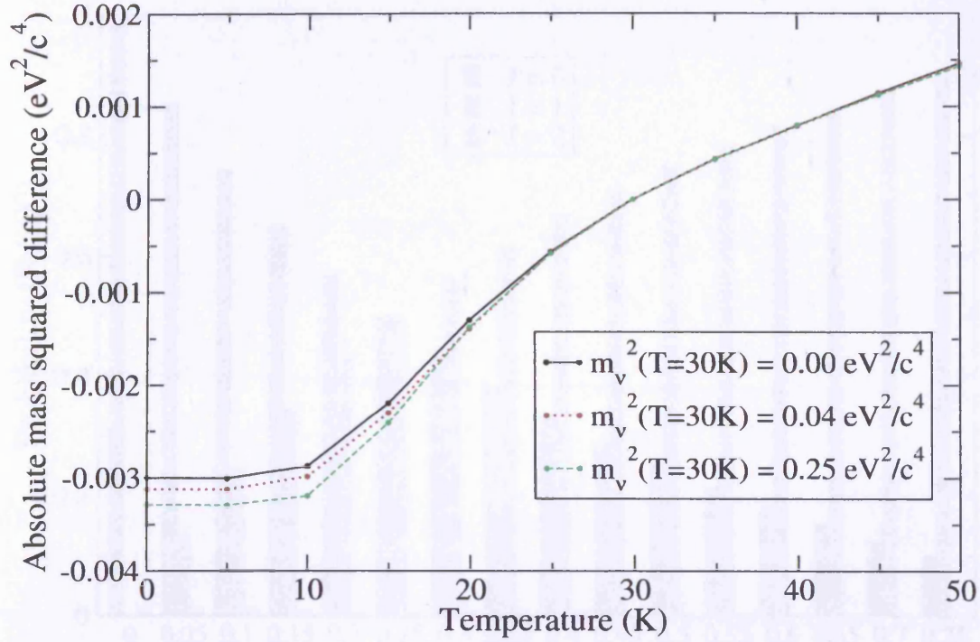
Figure 6.4: Error in the neutrino mass squared deduced from fitting, due to uncertainties in the source temperature (from fitting of \beta spectra with W_0 = 18.575 \text{ keV} and 100% T_2 ).
