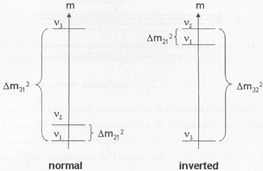
Figure 1.2: The normal and inverted hierarchy mass schemes for the neutrino masses.
