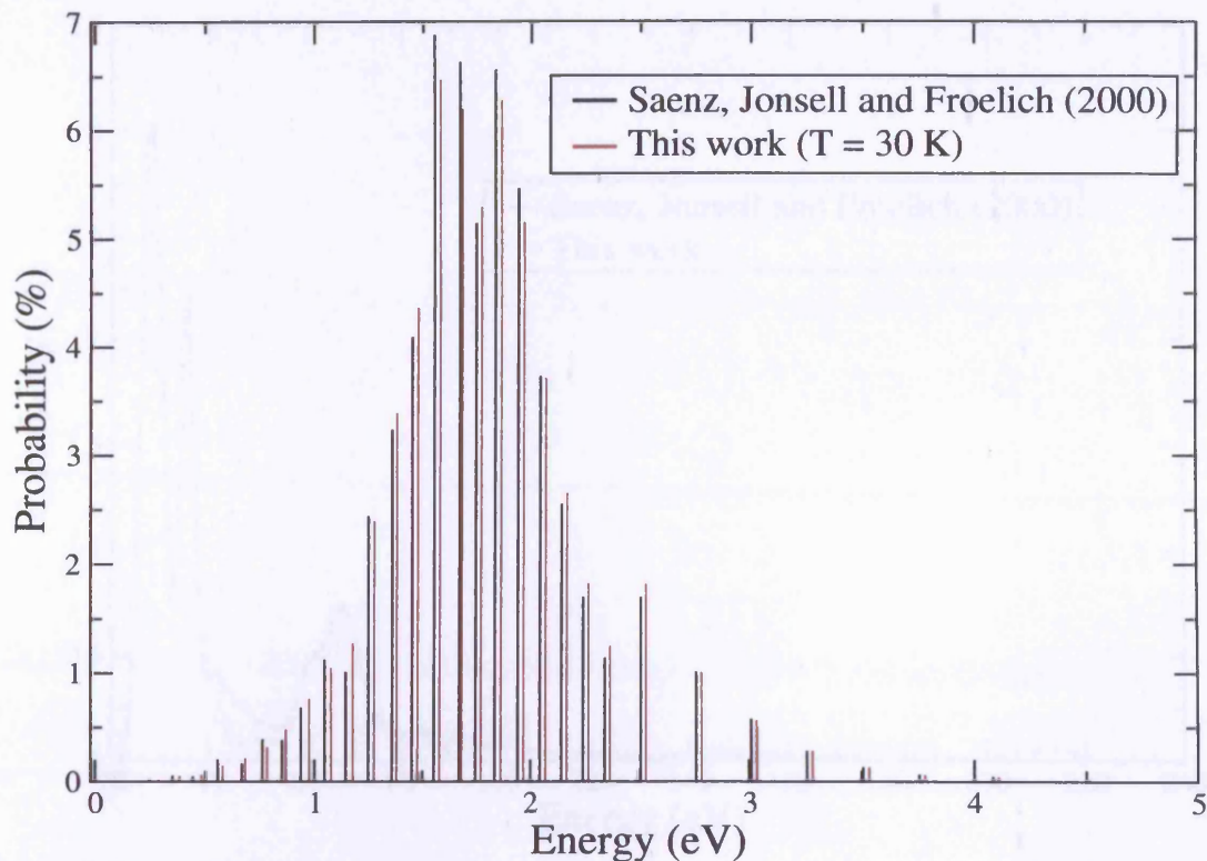
Figure 9.1: Comparison of the final state distribution of the electronic ground state of {}^3\text{HeT}^+ obtained in this work for a source temperature of 30 K with the FSD given in [106] for a source temperature of 0 K.
