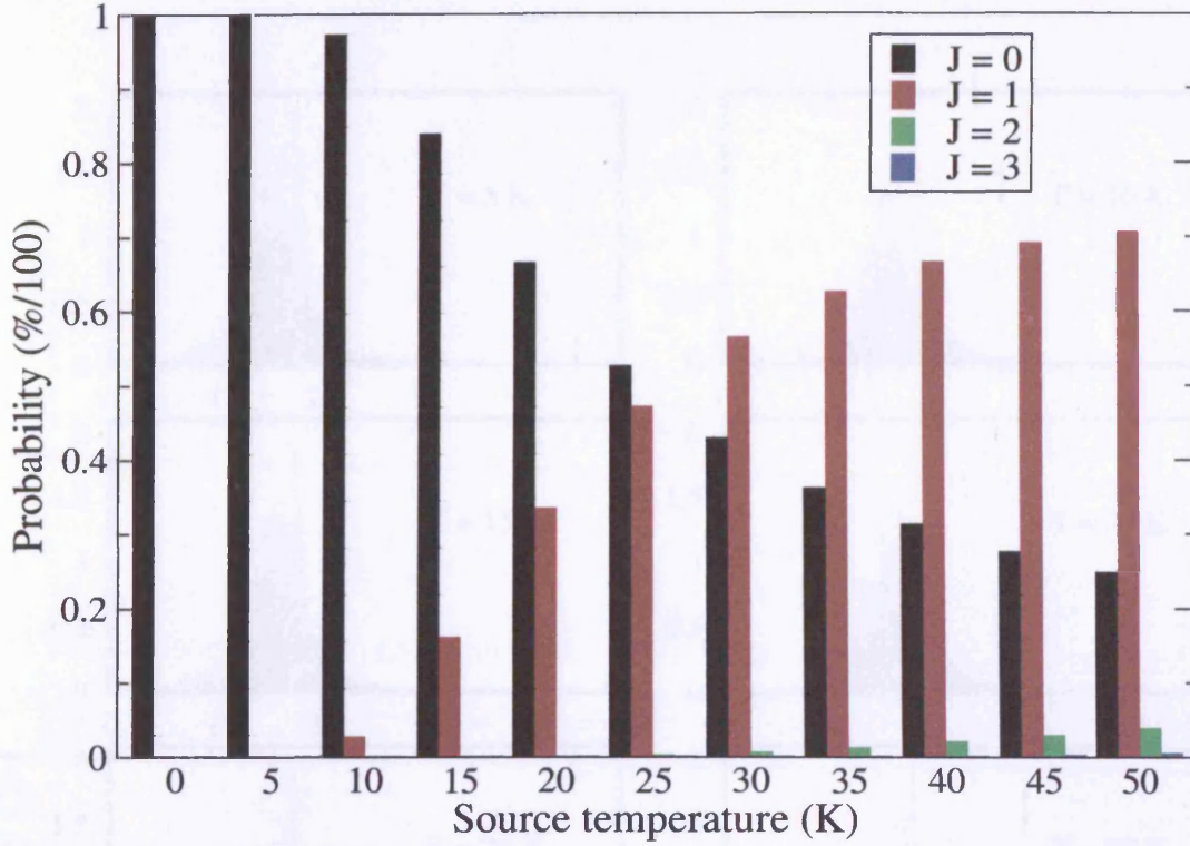
Figure 6.2: Distribution of T 2 molecules in each J state as a function of temperature
