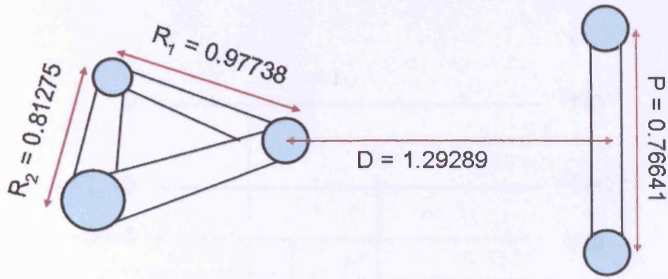
Figure 8.5: Global minimum structure for H_5^+
