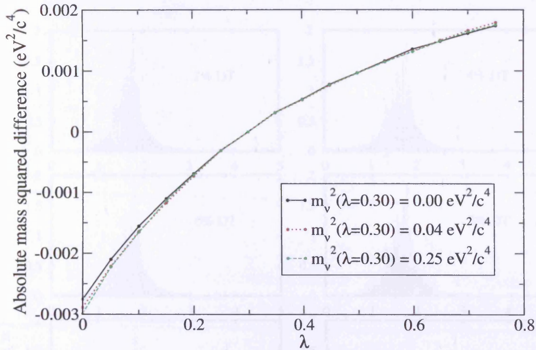
Figure 6.6: Error in the neutrino mass squared deduced from fitting, due to uncertainties in the ortho:para ratio (from fitting of \beta spectra with W_0 = 18.575 keV and 100% T_2 ).
