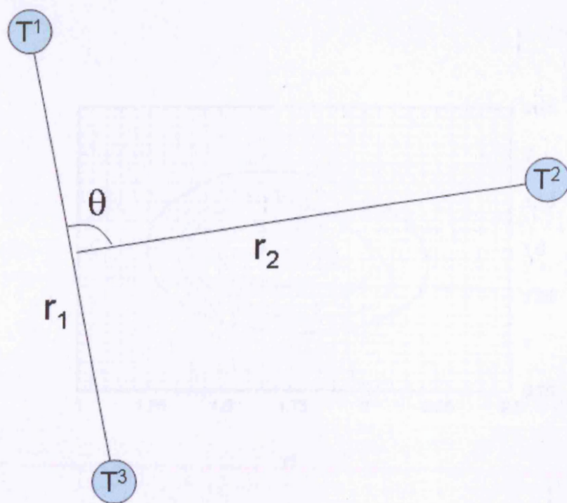
Figure 8.2: Jacobi coordinate system for T_3^+
