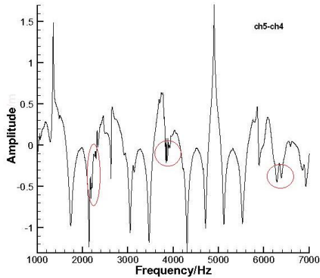
Figure 7 Signals of water pressure 1.765 MPa
