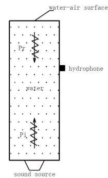
Figure 1 Sound velocity measurement principle
