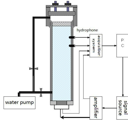
Figure 3 Sound velocity measurement system
