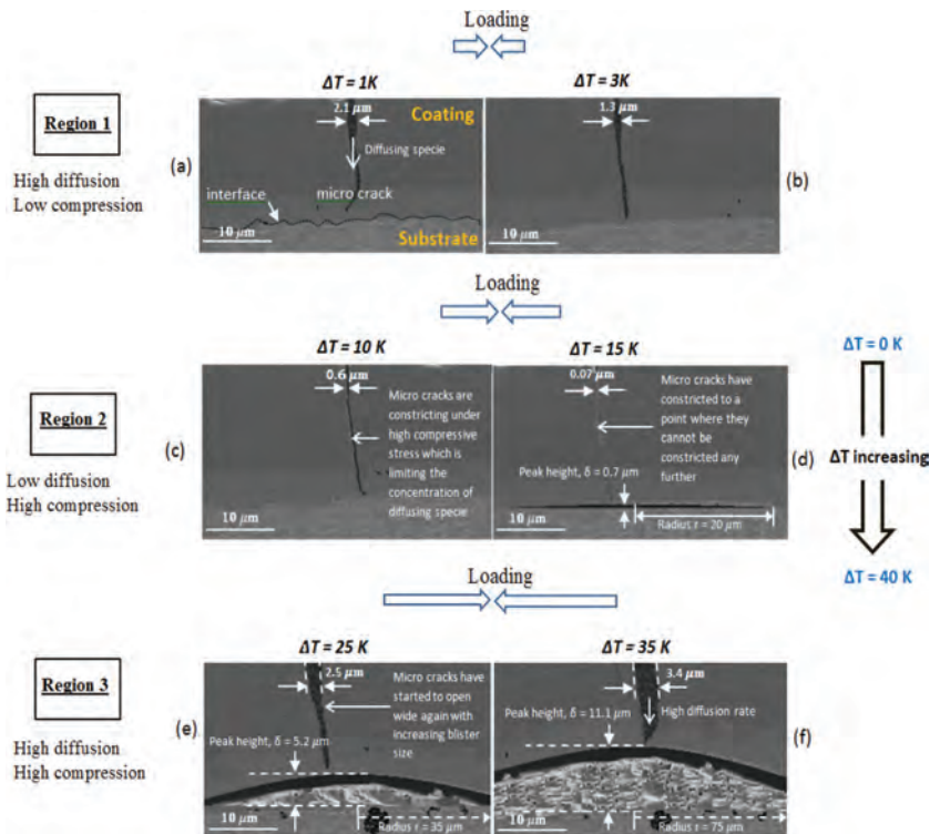
Figure 1: Samples micrographs at various temperature values [16].
