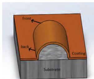
Figure 3: Schematic of straight-sided blister.
