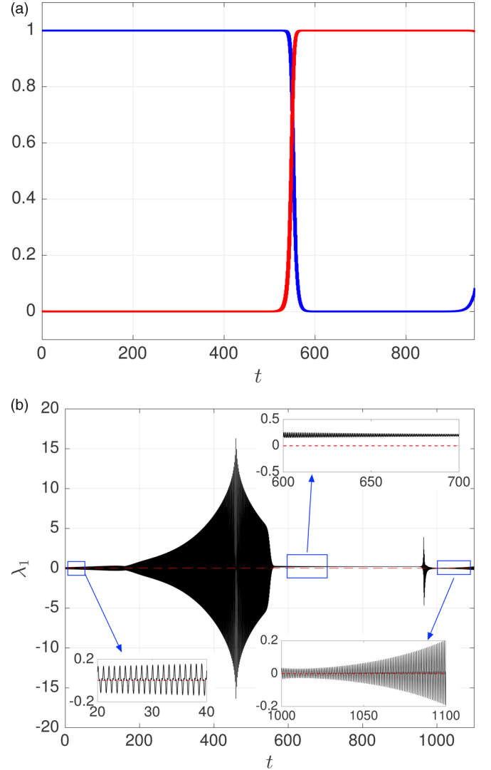
FIG. 4. (a) The evolution of \sqrt{v_{i,1}^2 + v_{i,2}^2} = \sqrt{1 - v_{i,3}^2} (blue) and v_{i,3} (red), where \mathbf{v}_i = (v_{i,1}, v_{i,2}, v_{i,3}) . (b) The evolution of the eigenvalue \lambda_1 as a function of time. The dashed red line marks \lambda_1 = 0 . Three closeup views are shown in the insets.
