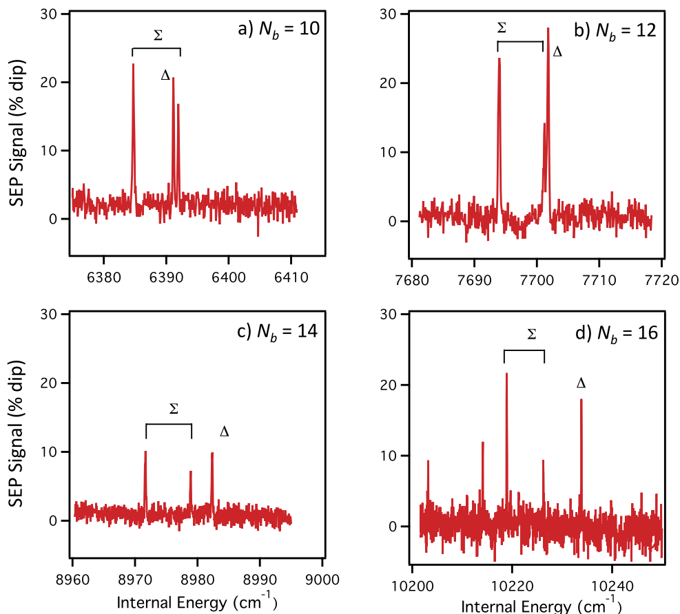
FIG. 2. SEP spectra of the lowest members of the N_b = 10 - 16 polyads. Transitions into the N_b = 10 and 12 polyads are recorded from Franck-Condon-active intermediate levels (using R(0) PUMP transitions). Transitions into the N_b = 14 and 16 polyads use Franck-Condon-forbidden levels as intermediates: the spectra of N_b = 14 are recorded from 3^1B^4, I , and those for N_b = 16 are recorded from B^4, I . The pattern of the \Sigma/\Delta splittings suggests that the state observed at 10218.9 \text{ cm}^{-1} is the N_b = 16 local-bender \Sigma state.
