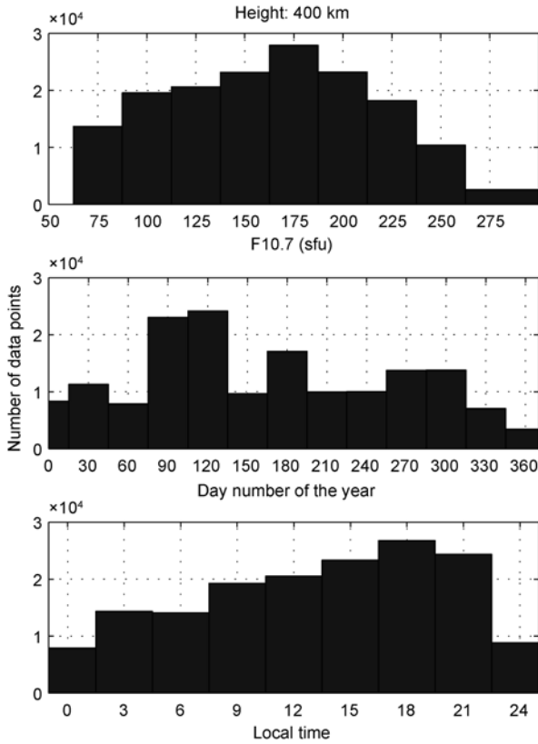
Figure 2 Data distribution for 400 km as a function of solar F10.7 index (top panel), day number of the year (middle panel), and local time (bottom panel).
