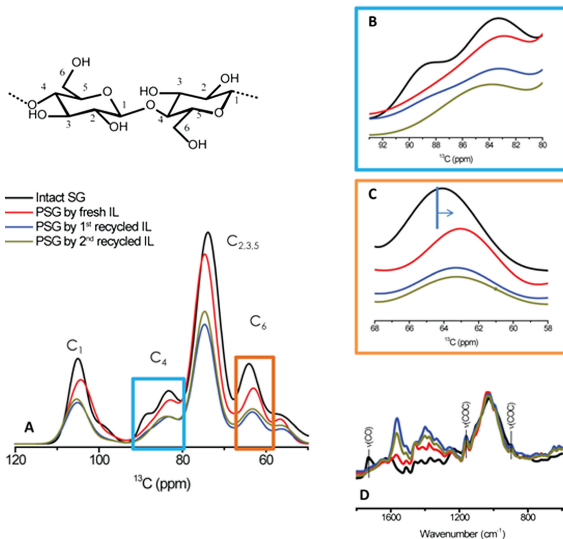
Fig. 5 Full CP/MAS 13 C NMR spectra ( \delta_{120-50} , a ), C 4 region ( \delta_{94-80} , b ), and C 6 region ( \delta_{68-58} , c ) of intact SG and PSG by fresh and recycled [C 2 C 1 Im][OAc] show that recycled [C 2 C 1 Im][OAc] can effectively
