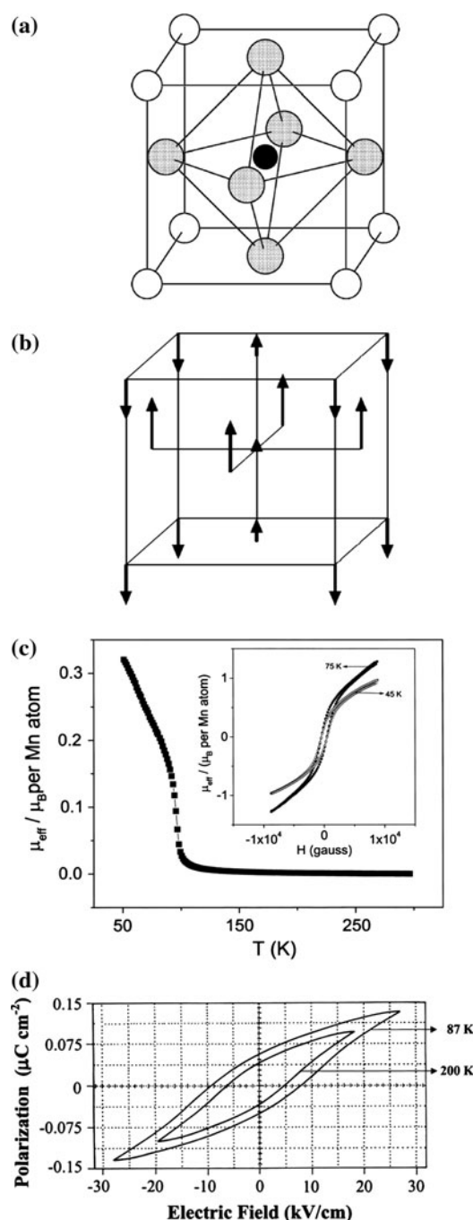
Fig. 11 a The perovskite structure of BiMnO 3 . Oxygen atoms are gray, Mn is black, and Bi is white [144]. b The Eigenvectors for one of the unstable gamma point phonon modes obtained through first-principles computations [144]. The opposite displacement of Bi and O create the possibility for ferroelectricity. c Measurements of the magnetic saturation at low temperature and d polarization versus electric field at 87 and 200 K [145]. Those measurements demonstrate the coexistence of ferromagnetism and ferroelectricity at low temperature. Reprinted Figure a and b with permission from [144]. Copyright 1999 by the American Physical Society. Figure c and d are reprinted from [145], copyright 2002, with permission from Elsevier
