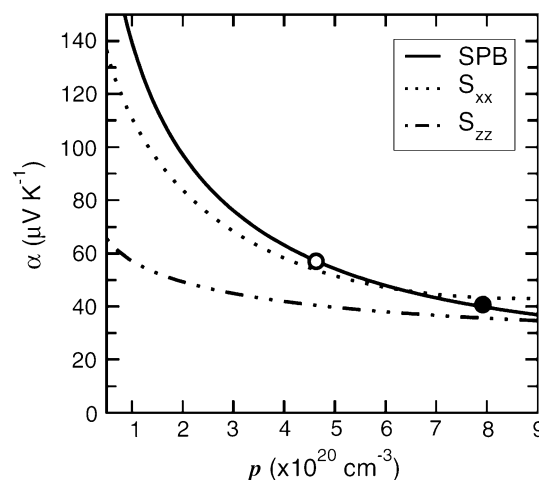
Fig. 8 Thermopower \alpha versus doping level for p-type LiZnSb. The circles represent experimental data measured by Toberer et al. [117] at 500 K, and the solid line represents a fit to the experiment using a single-parabolic band model. The thermopower predicted by Madsen et. al using first-principles calculations is shown as dotted and dashed-dotted lines [114]. The agreement between prediction and experiment indicates that it might be possible to screen for materials possessing a high thermopower through computation. Reprinted with permission from [117]. Copyright 2009, American Institute of Physics
