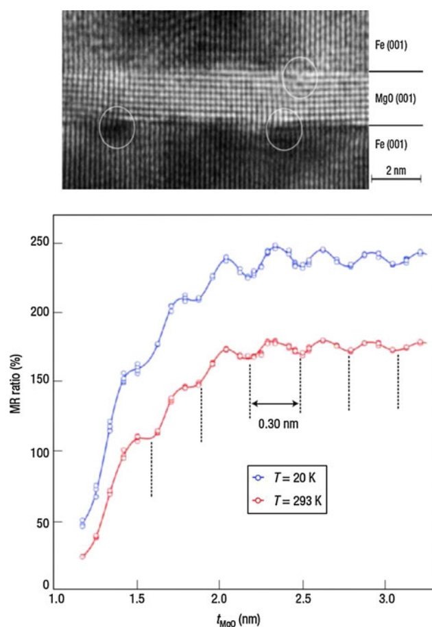
Fig. 10 High-resolution transmission electronic microscope picture of a Fe/MgO/Fe junction (the circles indicate dislocations) and TMR coefficient measurements in function of the MgO layer thickness [138]. The experimental measurement confirmed the very high TMR coefficient suggested by computations. Reprinted by permission from MacMillan Publishers Ltd: Nature Materials [138], copyright 2004
