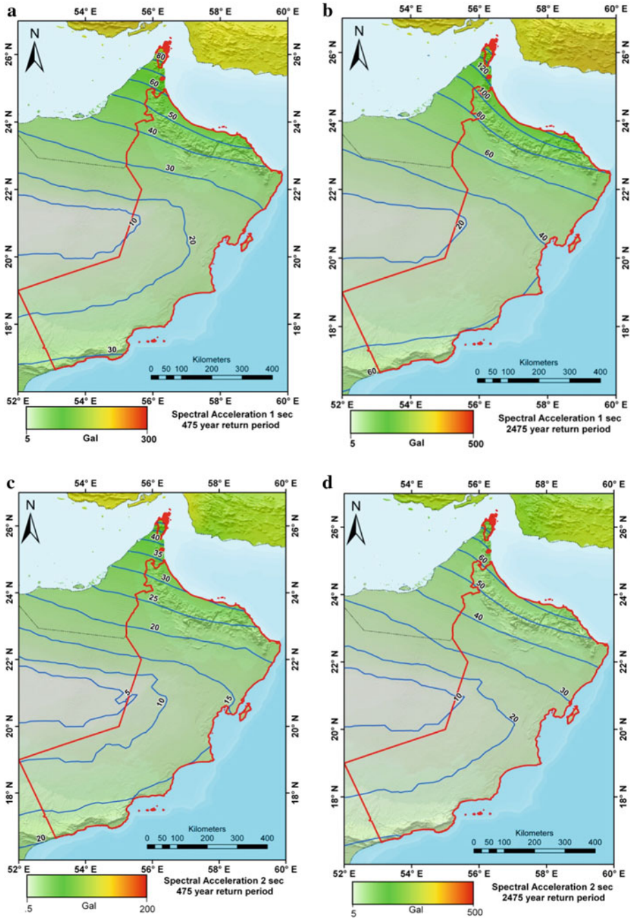
Fig. 15 Mean 1.0 s (a and b) and 2.0 s (c and d) spectral acceleration ( \text{cm/s}^2 ) on rock sites with 10 and 2 % probability of being exceeded in 50 years (475 and 2,475 years return periods) in the Sultanate of Oman
