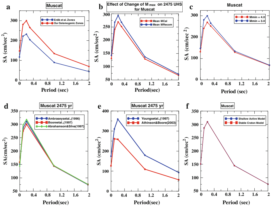
Fig. 19 Five percentage damped acceleration unified hazard spectra in \text{cm/s}^2 for a site in Muscat City; each panel evaluates the sensitivity to a specific input parameter of the hazard model: a seismogenic source model; b maximum magnitude; c minimum magnitude at Oman Mountains; d shallow seismic ground-motion prediction models; e subduction ground-motion prediction models; f stable craton ground-motion prediction models
