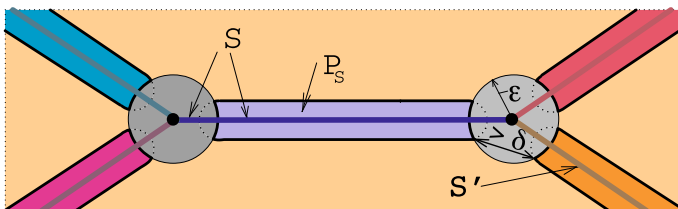
Fig. 4 For each stratum S , its approximation P_S lies within the \varepsilon -neighborhood of S . For every two incomparable strata S and S' , the distance between the sets P_S and P_{S'} exceeds \delta = \delta(\varepsilon)
