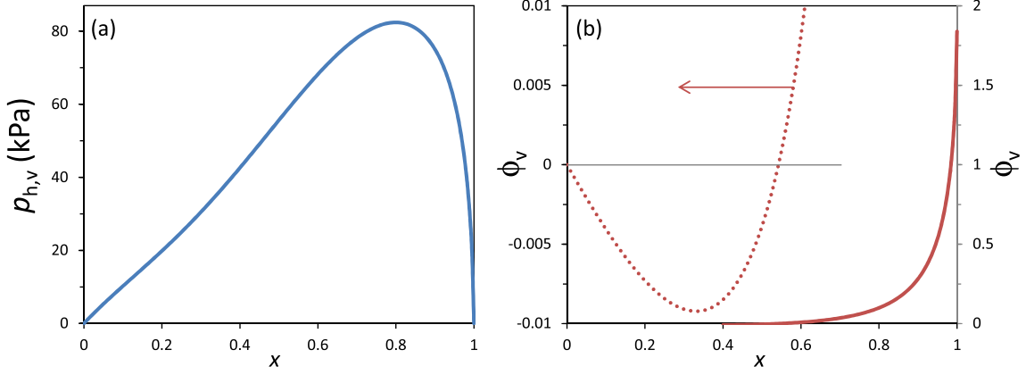
FIG. 3. Plots of (a) virtual hydrostatic pressure, p_{h,v}(x) , and (b) virtual electric potential, \phi_v(x) , vs axial position in pore, x . In (b) the dashed line is an enlarged view of the potential profile for x < 0.6 .
