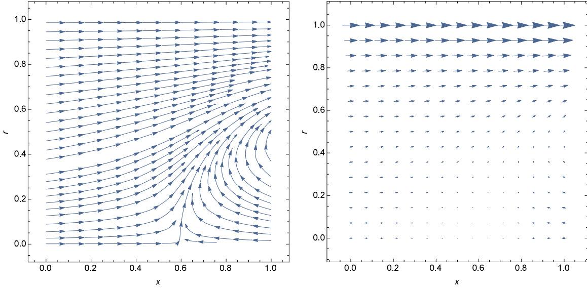
FIG. 4. Streamline (left) and vector field (right) plots of ionic current j_{\text{ch}}(x,r) . The streamline plot clearly demonstrates the inversion of j_{\text{ch}}(x,r) , while the vector field plot shows the higher magnitude of ionic current near the pore wall.
