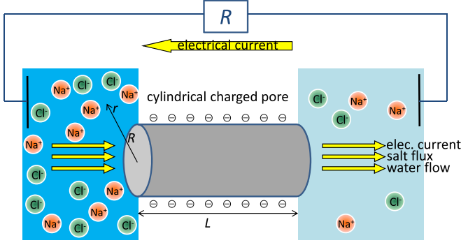
FIG. 1. Sketch of a charged cylindrical pore subjected to water flow, electrical current, and salt flux between a high-salinity (left) and low-salinity (right) reservoir.
