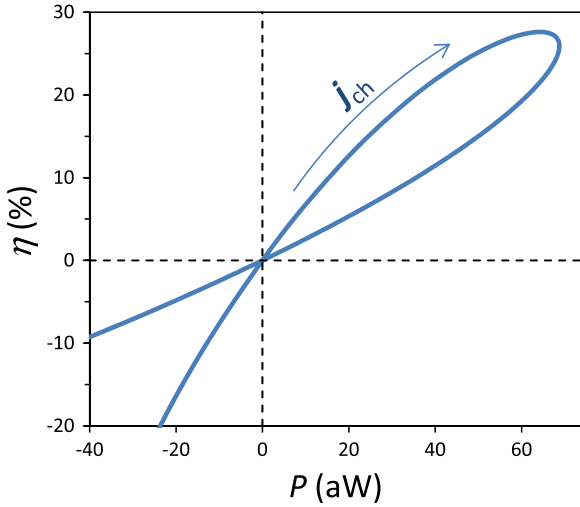
FIG. 5. Plot of energy efficiency \eta against generated electrical power P by a single charged nanopore placed between two electrolytes of different salinity ( c_{\text{ext}} = 10 and 100 mM). Current increases in direction of arrow.
