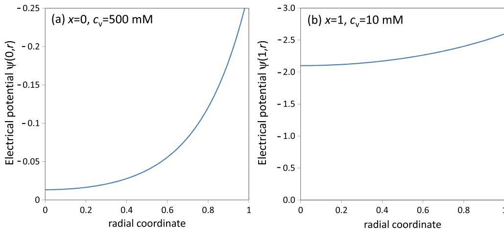
FIG. 2. Dimensionless electric potential \psi(0,r) and \psi(1,r) in a charged nanopore (radius R = 2 nm; surface charge \sigma = -10 mC/m 2 ) at the two ends of the pore, as a function of the dimensionless radial coordinate. At x = 0 , the potential drops off more quickly (relatively) from the wall towards the pore axis as the result of a higher c_{\text{ext}} .
