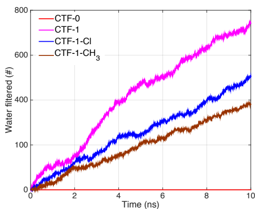
Figure 2 Water molecules filtered. The number of water molecules filtered for different CTF membranes is shown as a function of simulation time. The result shown in this figure is from a single simulation.
