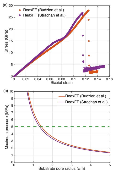
Figure 3 Mechanical properties of CTF-1 membranes. (a) The biaxial stress-strain curve and (b) the maximum hydraulic pressure as a function of substrate pore radius. The dashed-green line shown in (b) represents a typical RO pressure of 5 MPa.
