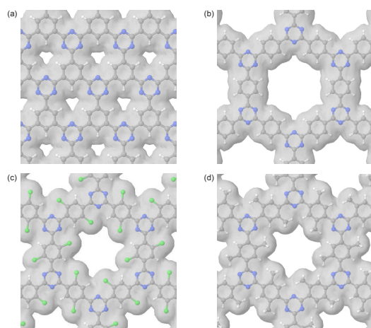
Figure 1 Atomic structure and pore shapes. The atomic structure and pore shape of (a) CTF-0, (b) CTF-1, (c) CTF-1-Cl, and (d) CTF-1-CH 3 . Colour code of grey: carbon, white: hydrogen, blue: nitrogen, and green: chlorine. Van der Waals surfaces are shown in transparent grey.
