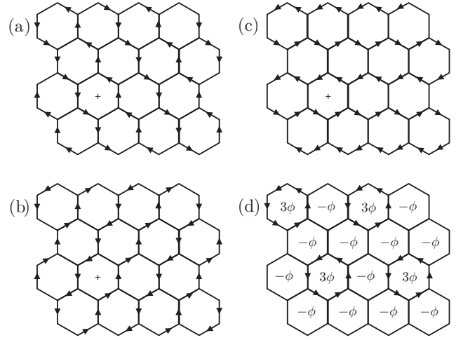
FIG. 8. Real-space picture of the honeycomb lattice flux order with F_2 symmetry. Figures (a)–(c) show the individual components as in Fig. 5 and (d) shows triple- M order. The pattern of fluxes is a direct analog of the triangular lattice as shown in Fig. 5(d).
