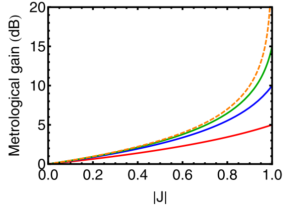
FIG. 3. (Color online) Spin squeezing using different couplings for state preparation and measurement. The solid lines show the metrological gain versus J for spin squeezed states with 15 dB, 10 dB, and 5 dB of squeezing (from above to below). The dashed line is the upper bound G for any squeezed state, where G = 1/[(1 - J^2)/2 + 1/S] . For J < 1 , the mismatch limits the maximum possible metrological gain.
