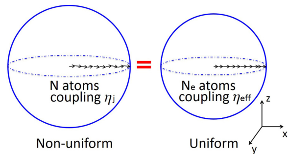
FIG. 1. (Color online) Equivalence between a system of N spins nonuniformly coupled to an optical mode and a slightly smaller uniformly coupled system of N_e spins. The equivalence is valid when the individual atomic spins are approximately aligned, |\langle \vec{S} \rangle| \approx Ns . The uniformly coupled system consists of N_e = N \langle \eta_j \rangle^2 / \langle \eta_j^2 \rangle effective atoms coupled with effective strength \eta_{\text{eff}} = \langle \eta_j^2 \rangle / \langle \eta_j \rangle , where \eta_j is the coupling strength for each atom j . Replacing the spin operators by effective spin operators (see text), within a wide range of parameters all dynamical properties are the same as those of the uniformly coupled system.
