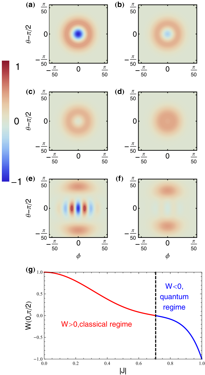
FIG. 2. (Color online) (a)–(d) The Wigner function [28] for the first Dicke state prepared and detected with different mode functions, for overlap parameter J = 1, \sqrt{2/3}, \sqrt{1/2} , and \sqrt{3/10} . (a) The center of Wigner function W(0, \pi/2) reaches -1 , the maximal allowed negative value, when we use the same nonuniform coupling for state preparation and readout, independent of the choice of the coupling. (b) If the preparation mode is a standing wave and the readout mode has uniform coupling, then J = \sqrt{2/3} , and W(0, \pi/2) is only -1/3 . (c)–(d) When J continues decreasing, the negative value of the Wigner function is smeared out due to the mismatch between state generation and readout. (e) For a squeezed cat state generated by a five-photons heralding event [13], the interference fringes still maintain the maximal visibility when J = 1 , regardless of the coupling of each atom. (f) The fringes are smeared out when J decreases (here J = \sqrt{2/3} ). (g) The dependence of W(0, \pi/2) on |J| for both states. All graphs are shown for atomic spin s = 1 and N = 2000 atoms.
