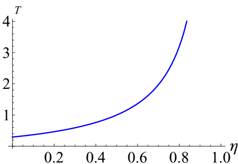
FIG. 3. (Color online) Tolerable excess noise N_T vs the transmissivity \eta for the reverse-reconciliation quantum data locking protocol, from Eq. (15). The asymptotic locked-key generation rate is nonzero for values of (\eta, N_T) below the curve.
