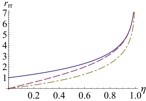
FIG. 2. (Color online) Achievable key rate for the pure loss channel ( N_T = 0 ) vs the channel transmissivity \eta , in bits per mode, for reverse reconciliation protocols. (Blue solid line) Achievable locked-key rate as from the expression in (14). (Red dashed line) Upper bound for the secret-key rate (assisted by two-way public communication), given by the expression in (2). (Yellow dash-dotted line) Achievable asymptotic secret-key rate according to the standard security definition as given by the reverse coherence information \log(\frac{1}{1-\eta}) [5].
