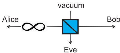
FIG. 5. (Color online) The lossy bosonic channel can be modeled as a beam splitter with transmissivity \eta and the environment mode initially in the vacuum state. In the first phase of the reverse reconciliation protocol, Alice sends one mode of a two-mode entangled state (denoted by the symbol " \infty ") down the channel.
