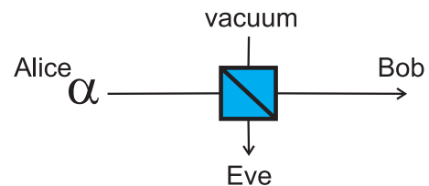
FIG. 4. (Color online) The lossy bosonic channel can be modeled as a beam splitter with transmissivity \eta and the environment mode initially in the vacuum state. In the direct reconciliation protocol, Alice sends coherent state down the channel.
