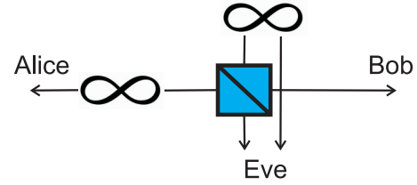
FIG. 6. (Color online) A scheme for an active Gaussian attack. The beam splitter mixes Alice's mode with one mode from an entangled pair (denoted by the symbol “ \infty ”). The eavesdropper Eve obtains both the modes of the two-mode state.
