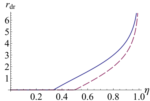
FIG. 1. (Color online) Achievable key rate for the pure loss channel ( N_T = 0 ) vs the channel transmissivity \eta , in bits per mode, for direct reconciliation protocols. (Blue solid line) Achievable locked-key rate as given by the expression in (13). (Red dashed line) Maximum fully unconditional secret-key rate, given by the expression \max\{0, \log(\frac{\eta}{1-\eta})\} [14].
