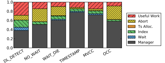
(b) Runtime Breakdown (512 cores)
