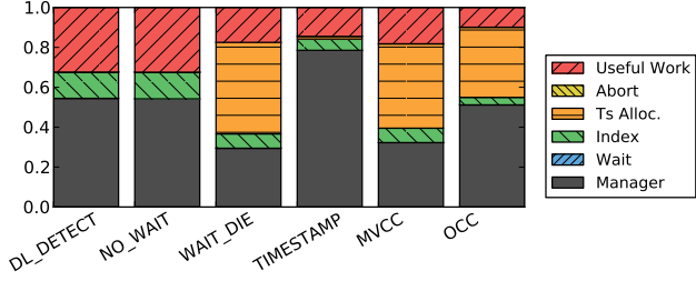
(b) Runtime Breakdown (1024 cores)
