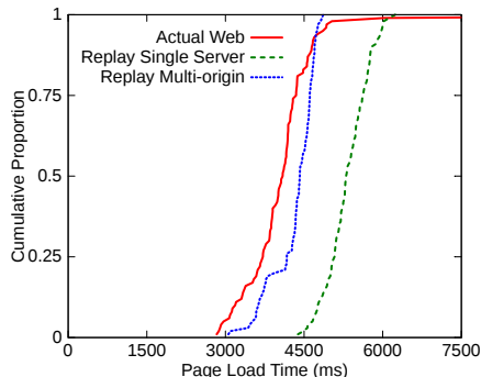
Figure 3: Multi-origin preservation yields measurements closer to the Web
