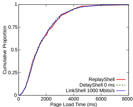
Figure 2: DelayShell's and LinkShell's low overhead
