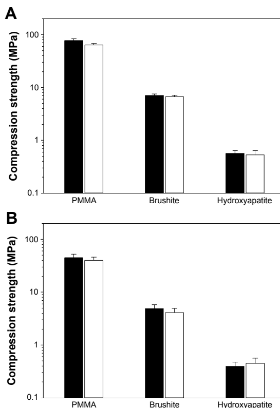
Figure 6 Compression strength of bone cements with 0% (control) and with organic nanoparticles (7% w/w for PMMA, 5% w/w for hydroxyapatite, and 1% w/w for brushite) freshly prepared (A), and after 7 days in PBS at 37°C (B).
