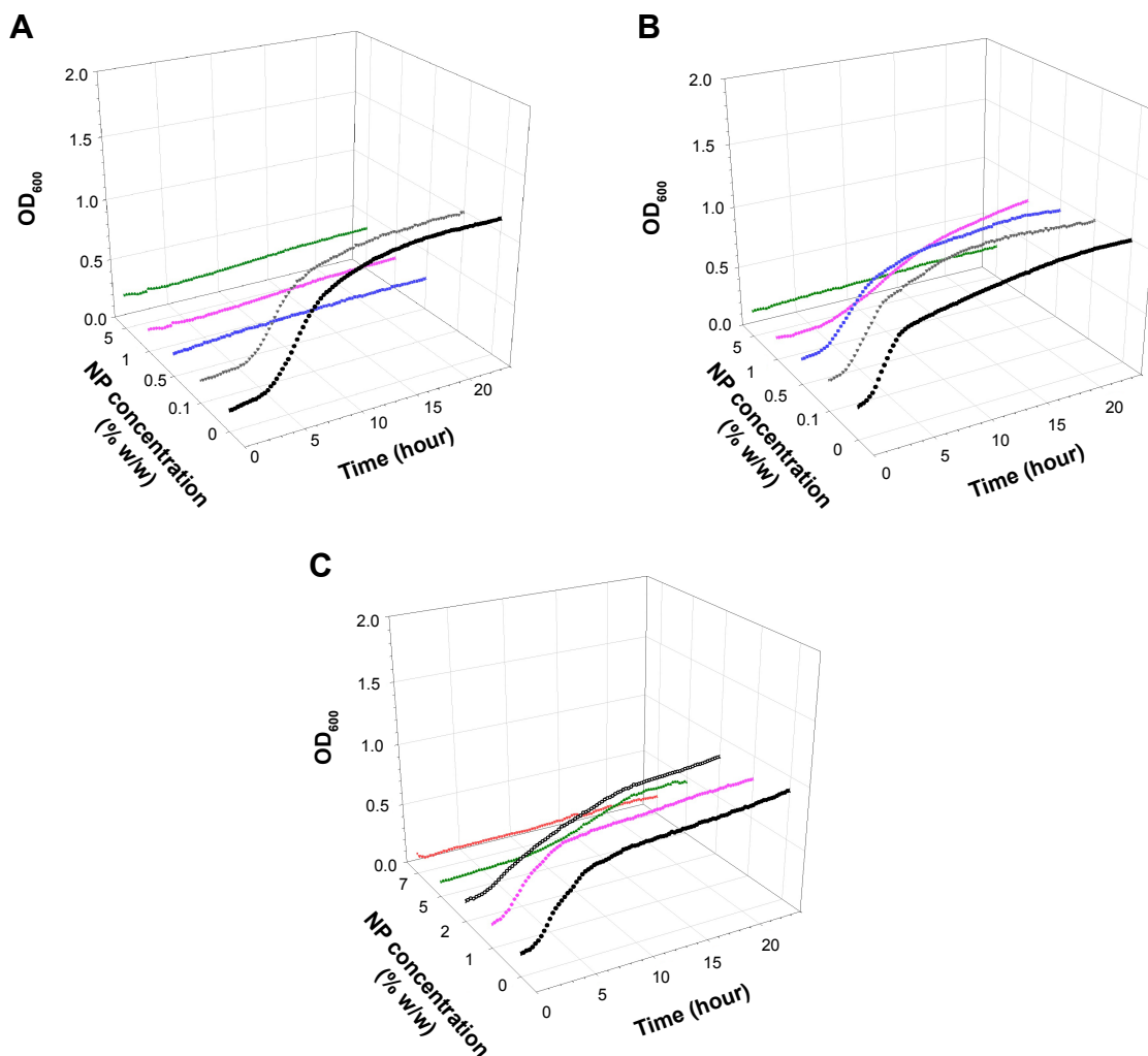
Figure 4 Examples of Staphylococcus epidermidis growth curves on (A) brushite, (B) hydroxyapatite, and (C) PMMA containing antimicrobial organic nanoparticles. Notes: ● 0%, ▼ 0.1%, ■ 0.5%, ◆ 1%, ○ 2%, ▲ 5%, ▼ 7%. Abbreviations: NP, nanoparticle; OD 600 , optical density at 600 nm; PMMA, poly(methyl methacrylate).
