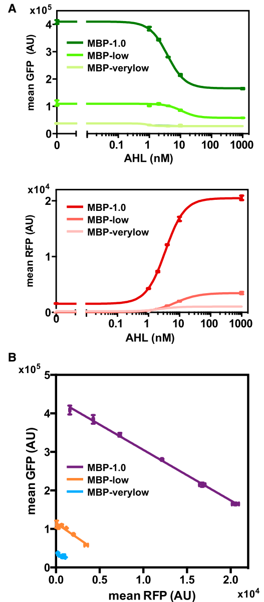
FIGURE 4 Influence of the plasmid copy number on the isocost line. (A) AHL dose response plots of GFP ( upper ) and RFP ( lower ) when plasmid copy number is changed. The plasmid MBP-1.0 was tested in the DIAL hosts JTK60 J ( 64 \pm 2 copies), H ( 18 \pm 4 copies), and E ( 4 \pm 1 copies). These copy numbers lead to 60%, 48%, and 29% change in GFP, respectively. (B) Linear relationships between GFP and RFP production. The steady-state values of GFP are represented as a function of the values of RFP in the same experiment. For numerical simulation results, see Section B4 in the Supporting Material . All plots represent mean values and standard deviations of populations in the steady state analyzed by flow cytometry in three independent experiments (for details, see Fig. S23 ).
