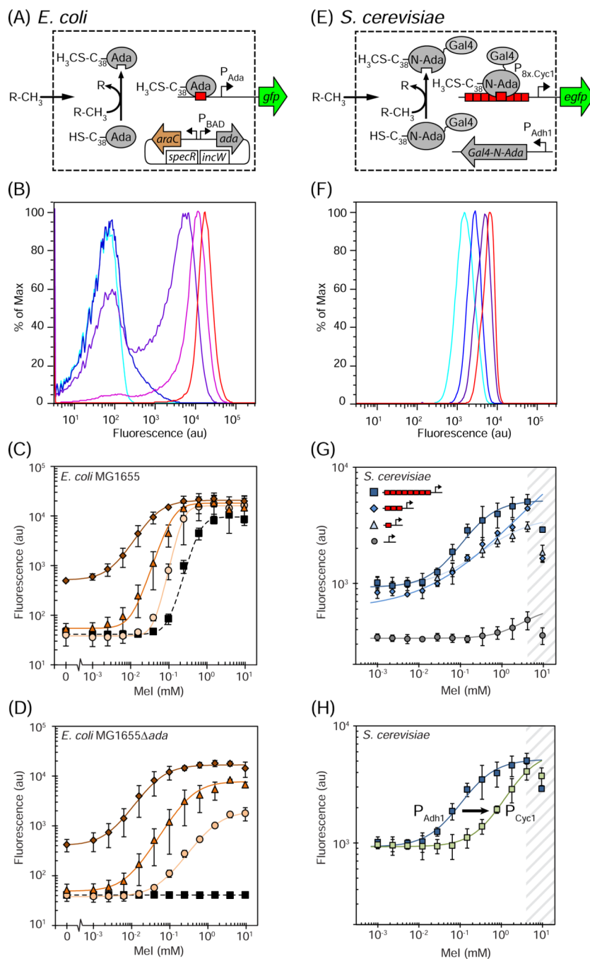
Figure 1. Mechanism and activity of E. coli and S. cerevisiae methylation sensors (A) Diagram of the E. coli methylation sensor. The Ada protein is expressed from either the genome or a low-copy plasmid (inset in lower right). (B) Overlaid histograms show the induction of E. coli MG1655 carrying the plasmid pFM45. The line colors correspond to different concentrations of MeI: 0 (light blue), 98 \mu M (dark blue), 244 \mu M (violet), 610 \mu M (pink), and 3.8 mM (red). (C) Response functions for the methylation sensor are shown in E. coli MG1655. Solid lines are strains expressing inducible Ada from plasmid pFM141 with variable amounts of arabinose: 0 mM (circles), 1 mM (triangles), and 10 mM (diamonds). E. coli containing only the reporter plasmid pFM45 is shown for comparison (black squares,
