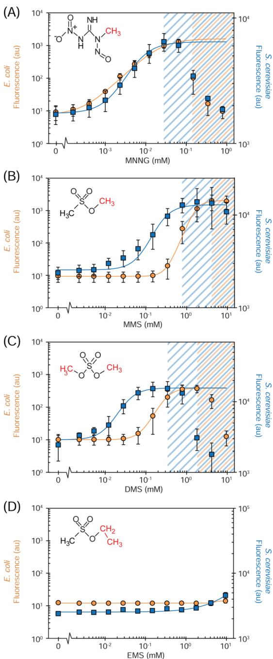
Figure 2. Response of the methylation sensors to S N 1 and S N 2 alkylating agents E. coli MG1655 carrying plasmid pFM45 and S. cerevisiae sensor P 8x.Cyc1 |P Adh1 were exposed to: (A) methyl nitronitrosoguanidine (MNNG), (B) methyl methanesulfonate (MMS), (C) dimethyl sulfate (DMS), and (D) ethyl methanesulfonate (EMS). E. coli (orange circles) and S. cerevisiae (blue squares) data correspond to the left and right axes, respectively. Insets are the structures of the respective alkylating agents, with the donated alkyl group highlighted in red. Blue and orange shaded regions indicate concentrations of alkylating agent higher than the LD 50 for S. cerevisiae and E. coli , respectively. The S. cerevisiae axis is scaled so that the highest and lowest values of the E. coli and S. cerevisiae
