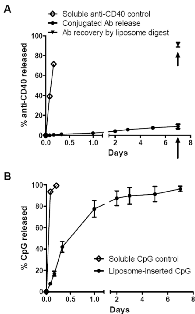
Figure 2. Controlled release of anti-CD40 and CpG from combination liposomes (filled symbols) by dialysis against serum-containing PBS in vitro , compared to the dialysis of freely soluble immuno-agonists (open symbols). (A) Release of conjugated anti-CD40 from combination liposomes, over 7 days of dialysis. On day 7, liposomes were disrupted with Tween 20 (arrow) and the amount of recovered anti-CD40 was measured. (B) Release of inserted CpG-lipid from combination liposomes, reaching a plateau after ~2 days.
