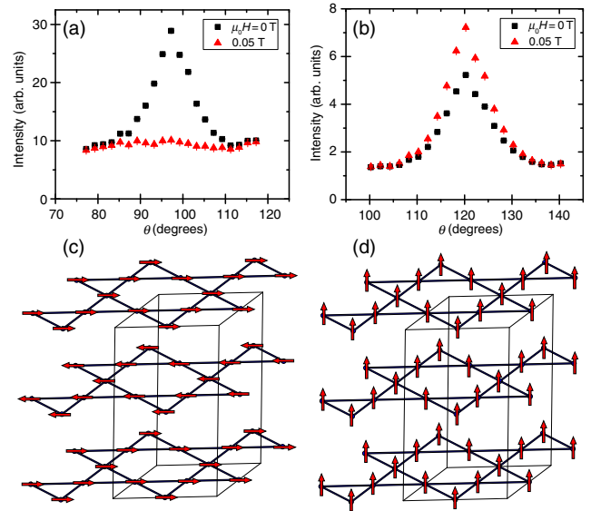
FIG. 2 (color online). Ground-state spin configuration of Cu(1,3-bdc). (a),(b) Elastic neutron scattering scans through the magnetic Bragg peaks measured at T = 70 mK at the (a) (0 0 1) and (b) (0 0 4) Bragg positions. Application of a magnetic field parallel to the kagome plane quickly suppresses the Bragg peak at (0 0 1) and increases intensity of the Bragg peak at (0 0 4) . (c),(d) Ground-state spin configuration of Cu(1,3-bdc), where spin-1/2 \text{Cu}^{2+} ions form a kagome lattice. (c) Zero magnetic field configuration. Spins within each plane are ordered ferromagnetically, and neighboring planes ordered antiferromagnetically. Spins point parallel to the kagome plane. (d) A small magnetic field can polarize and reorient all spins in the direction of the applied field. Here the field is applied perpendicular to the kagome plane.
