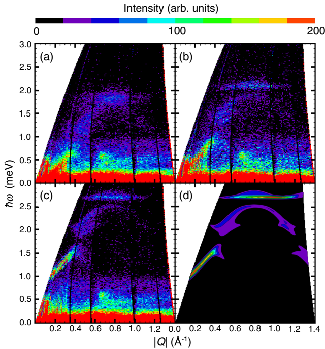
FIG. 3 (color online). Magnon dispersion in Cu(1,3-bdc). (a)–(c) Inelastic neutron scattering spectrum measured on LET with incident neutron energy 6.01 meV at T = 1 K and (a) zero field and applied fields (b) 2 T and (c) 7 T with the field applied perpendicular to the kagome plane. Black stripes are due to missing detectors. (d) Calculated inelastic structure factor for the Heisenberg ferromagnet with DM interaction convolved with the instrumental resolution function with parameters J = 0.6 meV, g_z = 2.2 , D_z = 0.09 meV, and \mu_0 H = 7 T, and displayed over the measurable range for the LET spectrometer. |\vec{Q}| is the magnitude of the momentum transfer vector parallel to the kagome plane.
