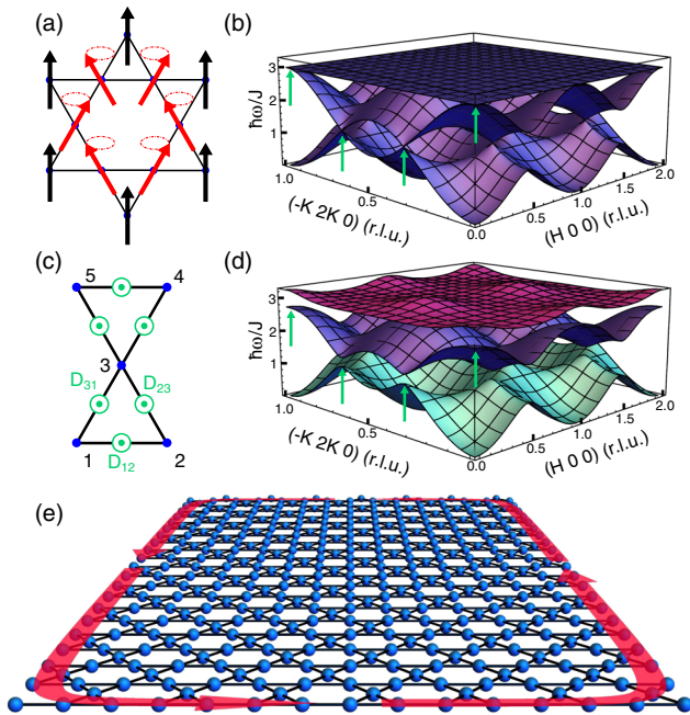
FIG. 1 (color online). Spin wave excitations in the kagome lattice ferromagnet. (a) A localized spin wave excitation supported by the kagome lattice. Because of the kagome geometry, excited (red) spins are decoupled from the rest of the lattice because a rotation of the neighboring ground-state (black) spins does not lower the overall energy of the spin configuration. Dashed lines indicate the excited spin precession path. (b) The spin wave dispersion of the kagome lattice ferromagnet, which consists of two dispersive modes and a perfectly flat mode, corresponding to the localized excitation shown in (a). Arrows show the locations of touch points between neighboring bands along [-K2K0] . (c) Out-of-plane component of the Dzyaloshinskii-Moriya (DM) vectors ( D_z ) on the kagome lattice, which have the same direction and magnitude for every bond because of the lattice symmetries. (d) Dispersion of the Heisenberg ferromagnet with DM interaction on the kagome lattice with D_z/J = 0.15 . Arrows are at the same locations as in (b) and show the gaps that open between bands due to the DM interaction. (e) Topologically protected chiral magnon edge modes. Magnons propagate around the edge of the lattice in a single direction.
