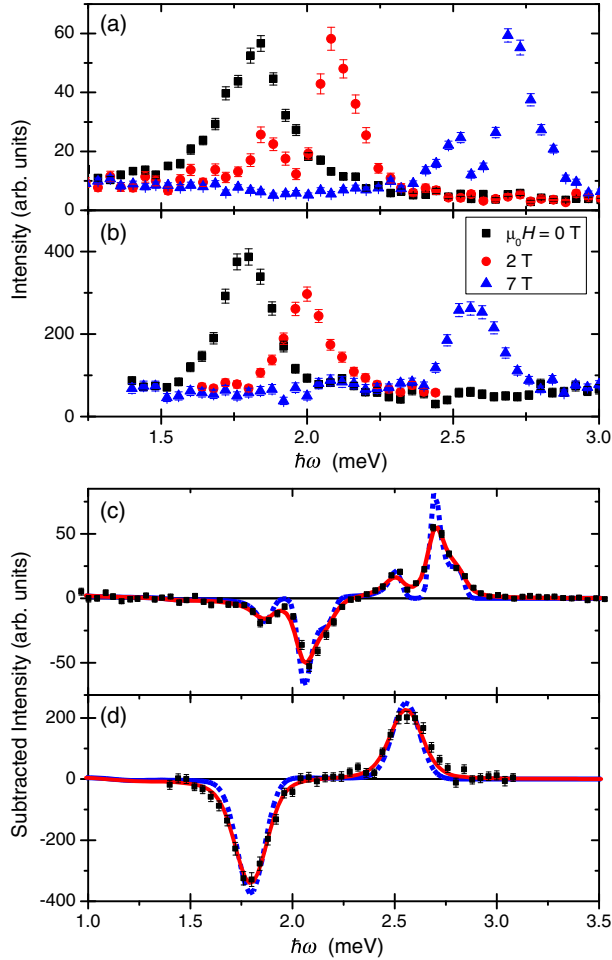
FIG. 4 (color online). Dependence of the magnon dispersion on the applied field direction. (a) Magnetic field applied perpendicular to the kagome plane. Data were taken on LET and integrated over the momentum transfer range 0.72 \text{ \AA}^{-1} \leq |\vec{Q}| \leq 0.88 \text{ \AA}^{-1} . (b) Magnetic field applied parallel to the kagome plane. Data were taken on SPINS at |\vec{Q}| = 0.8 \text{ \AA}^{-1} with a |\vec{Q}| resolution of \sim 0.15 \text{ \AA}^{-1} . (c),(d) Quantitative comparison to the deduced spin Hamiltonian. The data points in (c) correspond to the difference in intensities at \mu_0 H = 7 T and \mu_0 H = 2 T with the field perpendicular to the plane, and the data points in (d) correspond to the difference in intensities at \mu_0 H = 7 T and \mu_0 H = 0 T with the field parallel to the plane. The lines denote the calculated structure factor for the Heisenberg ferromagnet with DM interaction integrated over the same values of |\vec{Q}| as the data and convolved with the instrumental resolution function, assuming \delta -function spin waves (blue, dashed) and damped spin waves with damping \Gamma = 0.03 meV (red, solid). |\vec{Q}| is the magnitude of the momentum transfer vector parallel to the kagome plane. Error bars and uncertainty values throughout this manuscript are statistical in nature and represent 1 standard deviation.
