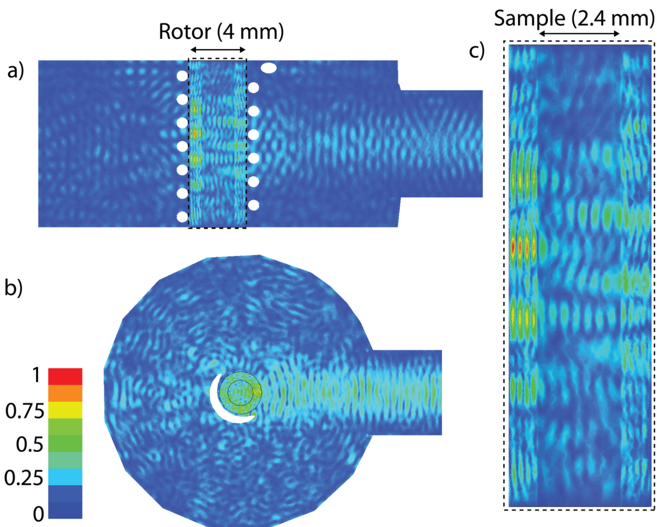
Figure 3. Normalized magnitude of B_{1S} , the transverse component of the microwave magnetic field, for the (a) vertical cross section of the probe, (b) the horizontal cross section of the probe and (c) the rotor and sample cross section. The magnitude \left(\sqrt{B_{1S} B_{1S}^*}\right) provides the maximum value of B_{1S} allowing for the observation of the standing wave patterns present in the input and the horizontal direction of the sample, as well as the interference fringes from the RF coil in the vertical direction of the sample.
