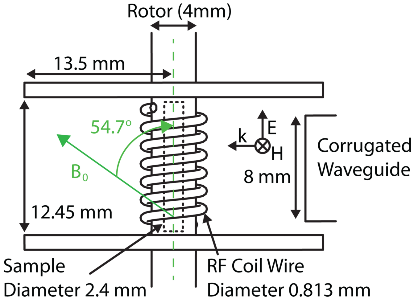
Figure 2. Cavity schematic as modeled in HFSS. The waveguide input is on the right.
