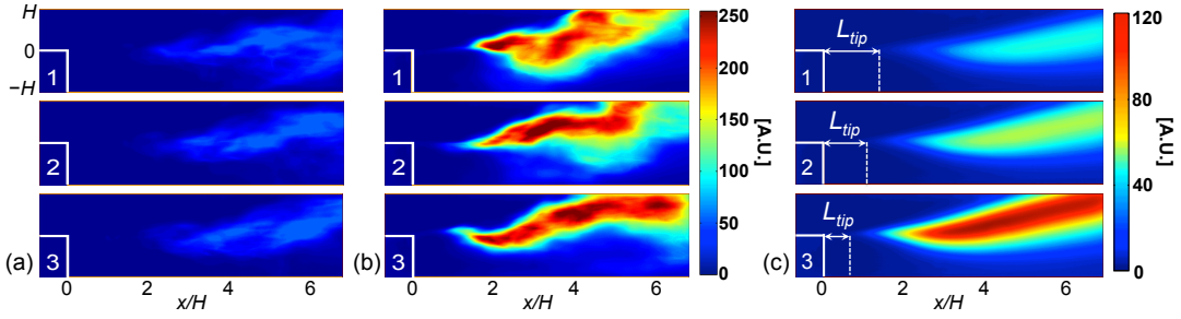
Figure 3: High-speed chemiluminescence images (4 ms between frames) are shown for (a) \phi = 0.75 and (b) \phi = 0.95 (both C_3H_8 /air flames), representative of Zone I and II, respectively. (c) The time-averaged chemiluminescence intensity contour at (1) \phi = 0.75 , (2) \phi = 0.79 and (3) \phi = 0.85 for C_3H_8 /air flames. The flame tip location ( L_{tip} ) is determined using the same absolute level ( \sim 4 a.u.). The field of view covers \sim 6.8 H downstream the step, where H denotes the step height, 20 mm.
