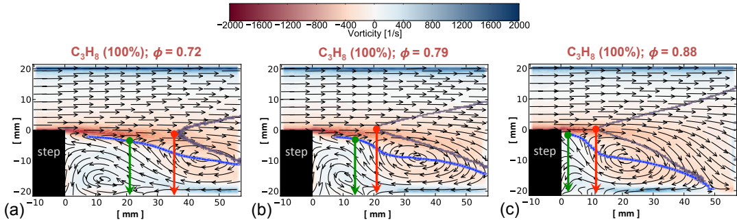
Figure 4: The time-averaged PIV data are shown for (a) \phi = 0.72 ; (b) \phi = 0.79 ; (c) \phi = 0.88 for C_3H_8 /air mixtures. The mean flame envelopes (lavender lines) are superimposed. The zero streamwise-velocity contours are indicated by blue lines. The axial locations of the saddle point and flame tip are marked by green and red arrows, respectively.
