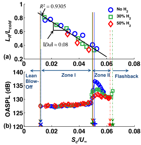
Figure 9: (a) The normalized reattachment lengths and (b) the OASPL (overall sound pressure level, see Eq. (1)), the same data shown in Figs. 8 and 2, respectively, as a function of the normalized consumption speed. A linear fit and the reciprocal of the slope is shown in (a).
