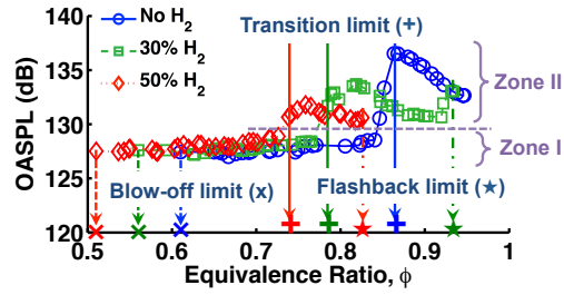
Figure 2: Overall sound pressure level as a function of equivalence ratio for different mixture compositions (indicated by volume) of C_3H_8/H_2 /air flames. T_{in} = 300 K and Re = 6500 for all cases.
