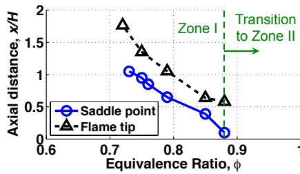
Figure 5: The axial locations of the saddle point and flame tip estimated over a range of \phi for C_3H_8 /air mixtures.
