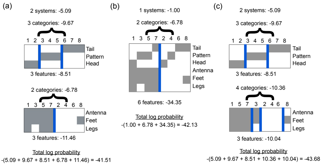
Figure 5. Three possible solutions to the 3/2 data. The solutions correspond to (a) the best solution, (b) a simpler solution that accounts for the data less well, and (c) a solution that accounts for the data better, but at the cost of greater complexity.
