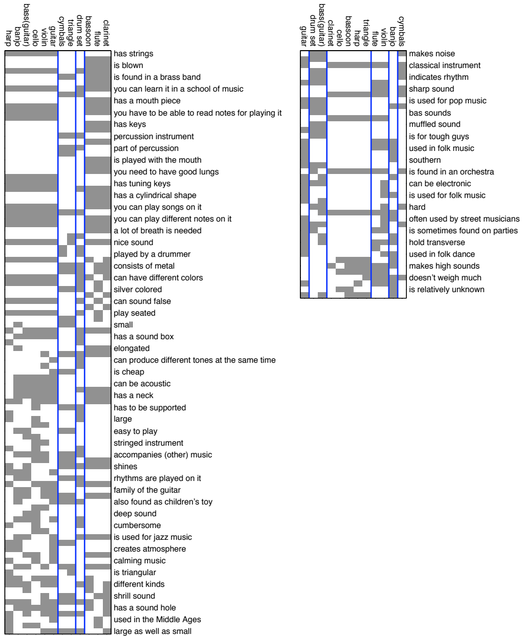
Figure 10. The best solution found by CrossCat for the instruments data, containing two systems of (a) taxonomic, and (b) social use categories. The system of taxonomic categories includes wind, percussion, and string instruments. The system based on social use includes categories of classical instruments such as cello, harp, bassoon, and clarinet, and the rhythm section (drums and bass) of rock bands are grouped.
