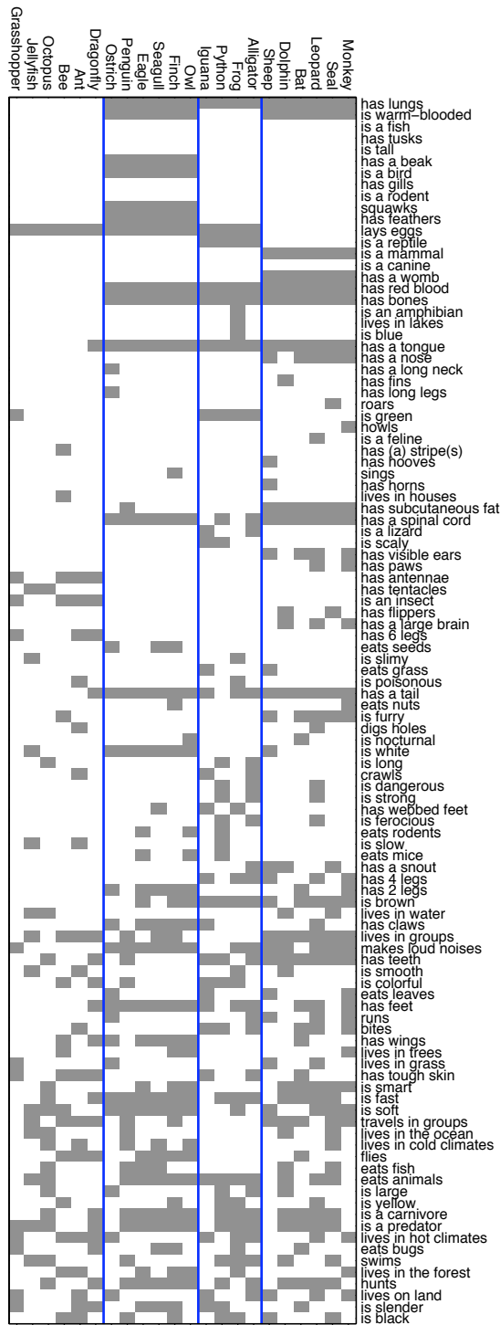
Figure 2. The best solution to the animals data according to the single system model. The model finds four intuitively compelling categories: mammals, invertebrates, birds, and reptiles/amphibians. Features are sorted from those that are best explained by these categories to those that are most poorly explained. Note that while many features such as “has lungs” are well explained, many that seem structured, such as “is a carnivore” are not.
