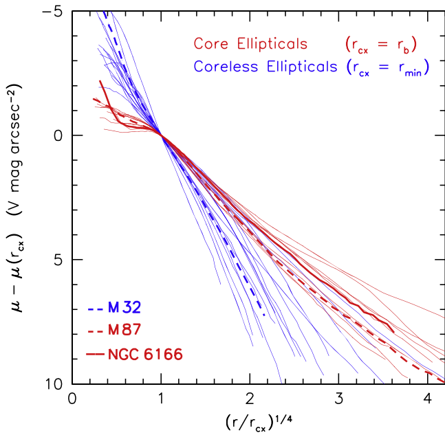
Figure 12. Major-axis profiles of all KFCB elliptical galaxies scaled together in radius and surface brightness. Core ellipticals are scaled at r_{cx} = r_b , the break radius given by the Nuker function fit in Lauer et al. (2007). Coreless ellipticals are scaled at the minimum radius r_{min} that was used in the KFCB Sérsic fits; inside this radius, the profile is dominated by extra light above the inward extrapolation of the outer Sérsic fit. NGC 6166 and the fiducial galaxies M87 and M32 are plotted with thick lines. There is no sign of two-component structure in NGC 6166; its profile resembles those of other core galaxies. That is, the cD halo is not distinguishable using photometry alone.
