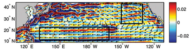
FIG. 1. The time-mean small-scale zonal velocity (color; \text{m s}^{-1} ) and the direction of the large-scale time-mean velocity (vectors) on the time-mean 1025.6 \text{ kg m}^{-3} isopycnal from the ECCO2 state estimate. Black boxes denote the CNP and ENP regions. Here, time-mean denotes the temporal average over the years 1992–2007, large scale means the 4^\circ \times 4^\circ running average, and small scale is the deviation from the large scales.
