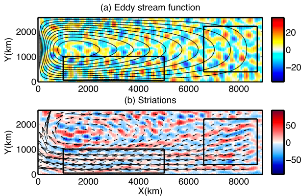
FIG. 10. Snapshots of the (a) eddy streamfunction \psi ( 10^3 \text{ m}^2 \text{ s}^{-1} ) and the (b) part of zonal eddy velocity with frequencies lower than \Omega_S ( 10^{-3} \text{ m s}^{-1} ) in Exp2. Black contours illustrate the subtropical gyre, and black boxes denote the central and east regions. Vectors denote eddy propagation velocities diagnosed using the method in appendix A. As a reference, the maximum value of these propagation velocities in the domain shown here is 0.1 \text{ m s}^{-1} .
