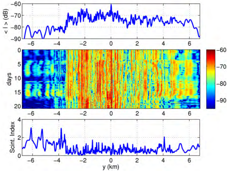
Fig. 4. Center panel: The model intensity I(y,t) at range x=12 km and depth z=128 meters depth in plotted. Upper panel: The mean over time is plotted. Lower panel: The scintillation index is plotted as a function of y . The scintillation index is the intensity variance divided by the mean intensity squared.
