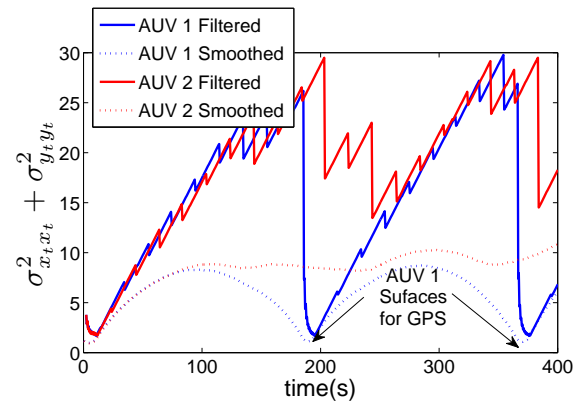
Fig. 7. The instantaneous (filtered) and smoothed uncertainties of two vehicles cooperatively localizing using the proposed method. AUV 1 surfaces for GPS twice thus bounding the uncertainty for both vehicles.
