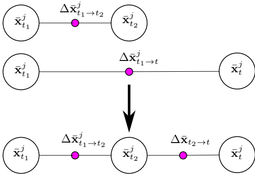
Fig. 4. The subtraction property illustrated on the change of position factors. The top two change in position factors are received and are decomposed into the single bottom position chain.
