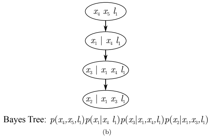
Figure 3: Example Bayes tree structures produced by eliminating the same factor graph from Figure 1 using the two different variable orderings from Figure 2.
