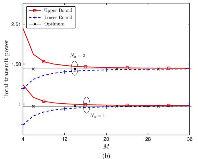
Fig. 4. Total transmit power based on asymptotically optimal algorithms as a function of the (a) NUSS and (b) parameter M for networks with eight anchors and one/two agents: (a) M = 4, 8, 16 ; (b) NUSS = 0.15.
