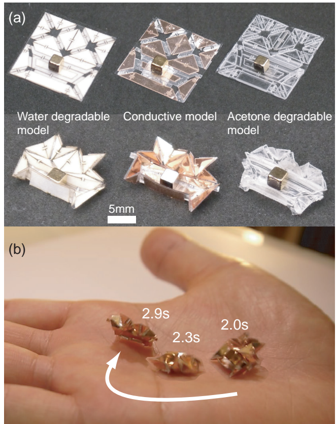
Fig. 1: The developed origami robot. (a) (From left to right) water-degradable model whose outer layer dissolves in water; conductive model (aluminum coated polyester); acetone-degradable model whose entire body (except magnet) dissolves in acetone. (b) Self-folded robot (controlled by a magnetic field) walking on a palm.
